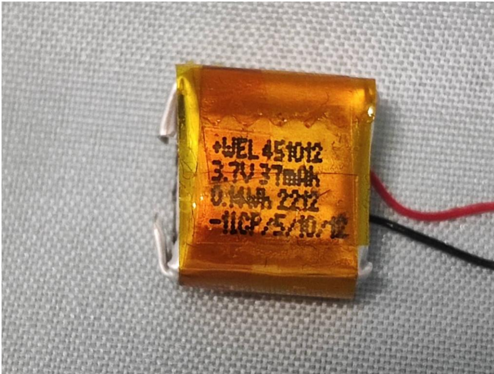
(17) EUT Photo_Right Ear (Battery: WeAction)
