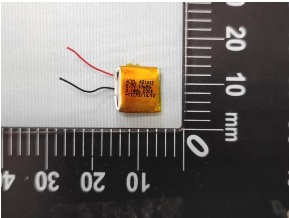
(18) EUT Photo_Right Ear (Battery: Golden CEL)
