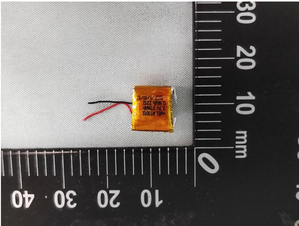
(6) EUT Photo_Left Ear (Battery: WeAction)
