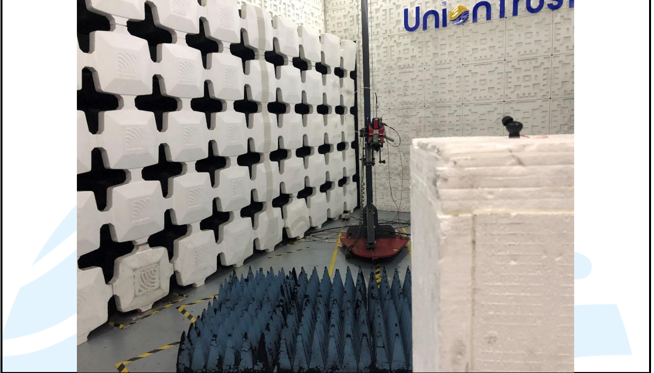
Radiated emission Test Setup (Above 1 GHz) -Left
