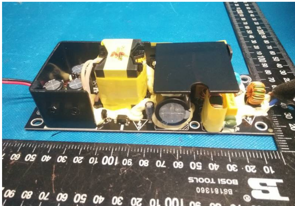
Fig. 9: Power board top view_2 (in both active speaker and passive speaker)
