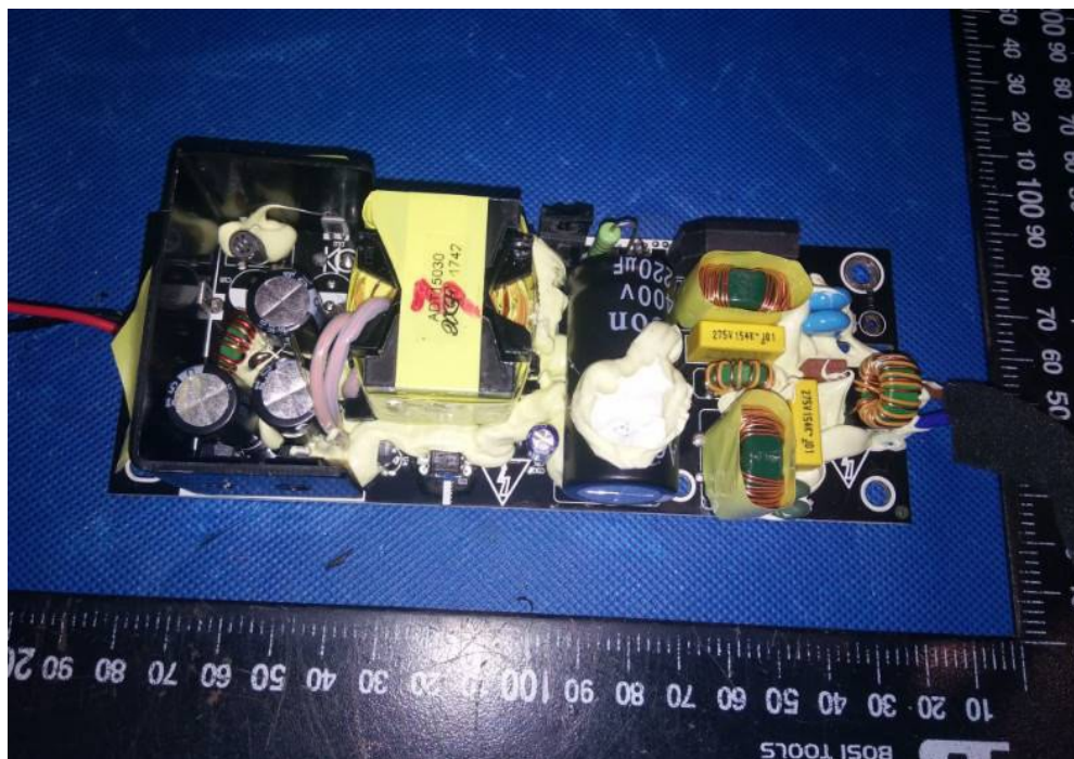
Fig. 10: Power board bottom view (in both active speaker and passive speaker)
