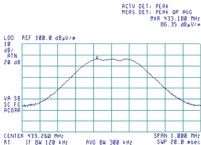
Plot 7.3.2 Radiated emission measurements at the fundamental frequency 433.26 MHz
