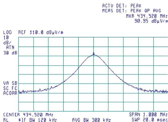
Plot 7.2.16 Radiated emission measurements at the fundamental frequency 434.52 MHz, UHF3 transmitter
