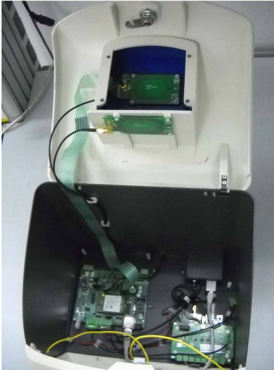
Photograph No.1 StockBox system internal view
