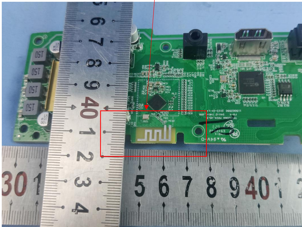
BT Antenna
