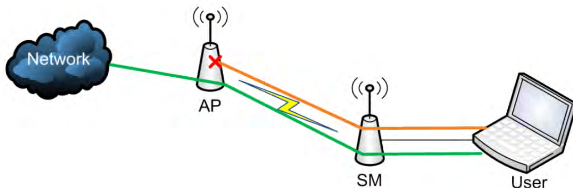
Figure 31: RF Telnet Access Restrictions (orange) and Flow through (green)
