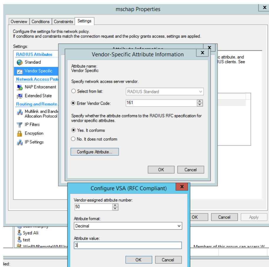
Figure 75: RADIUS VSA configuration
