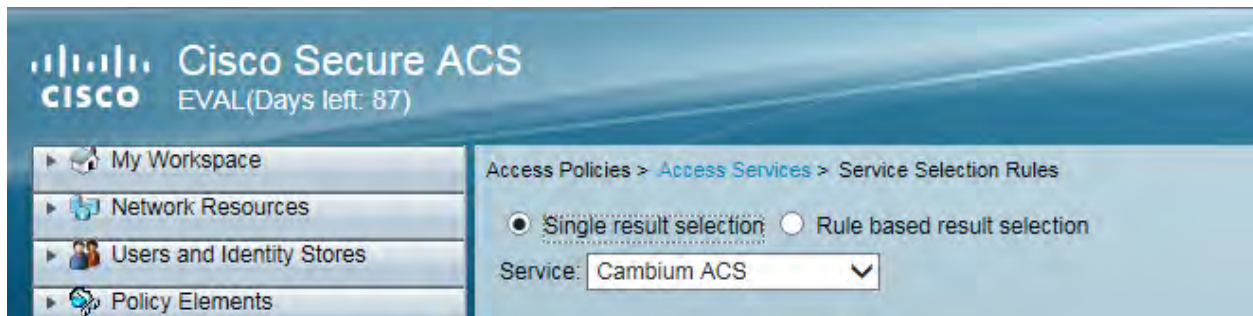
Figure 80: Service selection
