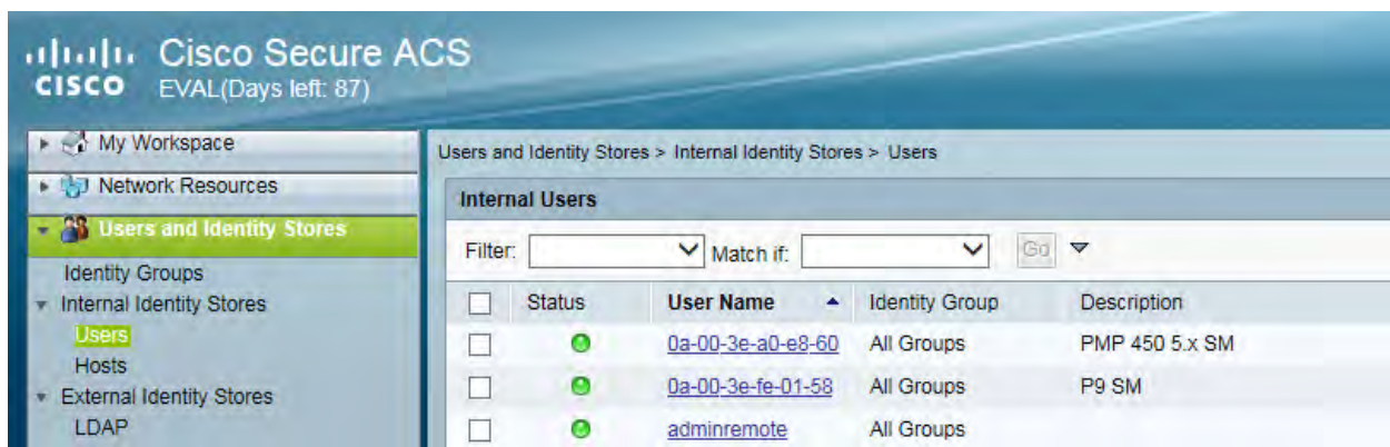
Figure 77: Creating users
