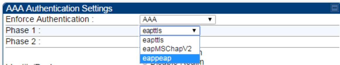
Figure 71: EAPPEAP settings
