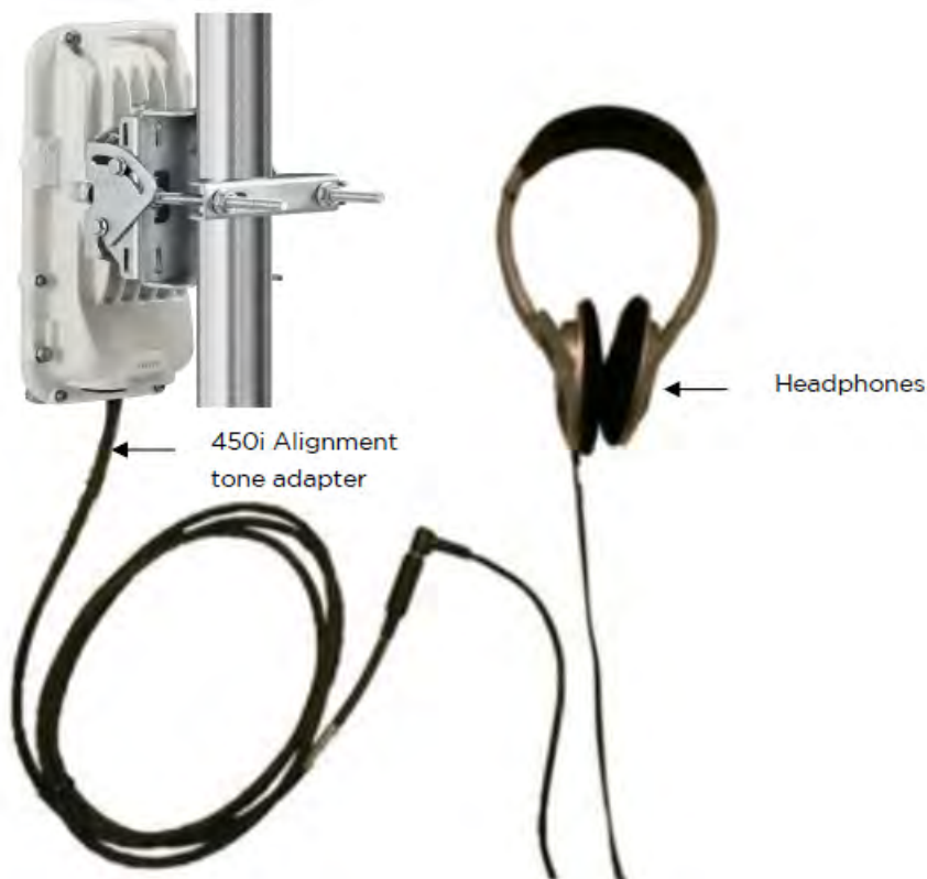
Figure 91: PMP/PTP 450i Series link alignment tone
