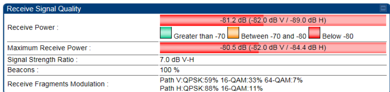
Figure 89: Alignment Tool tab of SM – Receive Power Level < -80 dBm
