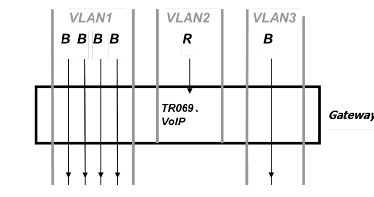
Figure 4 Multi VLAN
