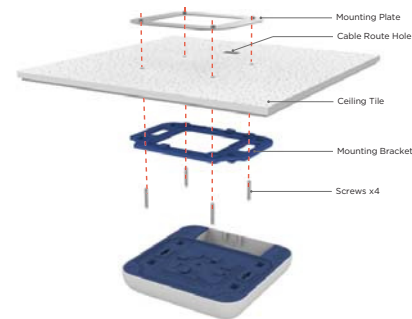
Exploded View
