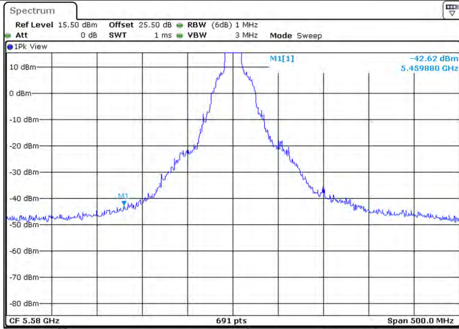
Plot on Configuration VHT20 / 5580 MHz / Peak / Port 2 (TX2)
