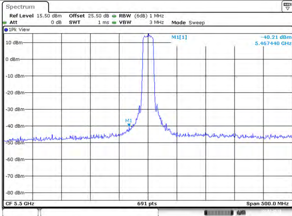
Plot on Configuration VHT20 / 5500 MHz / Peak / Port 1 (TX1)
