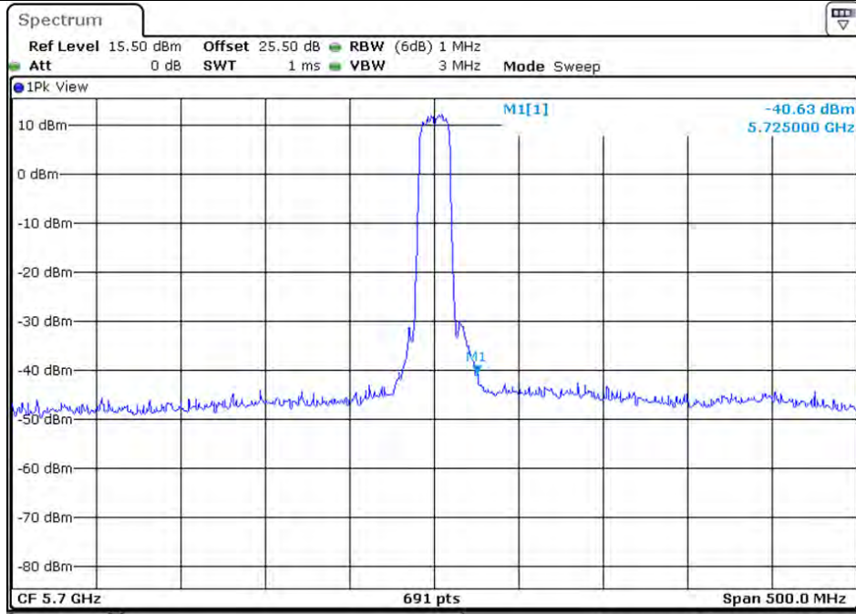
Plot on Configuration VHT20 / 5700 MHz / Peak / Port 2 (TX2)
