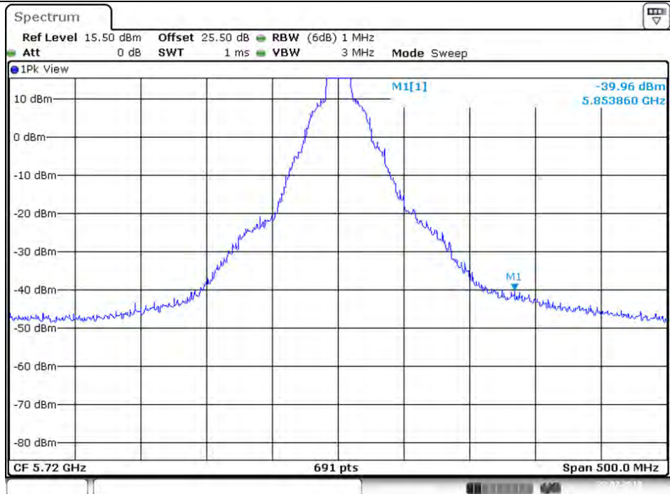
Plot on Configuration VHT20 / 5720 MHz / Peak / Port 2 (TX2)
