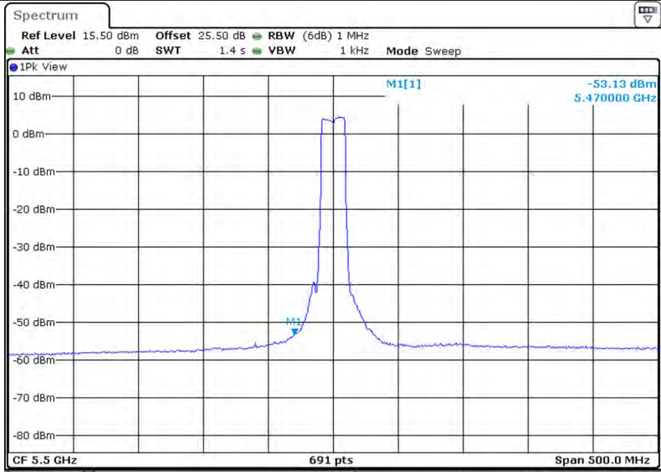
Plot on Configuration VHT20 / 5500 MHz / Average / Port 2 (TX2)
