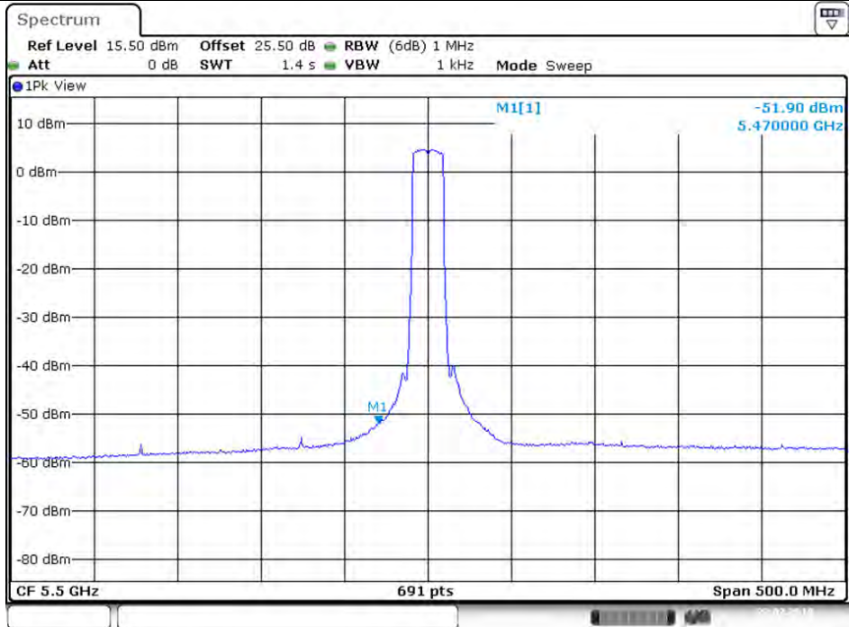
Plot on Configuration VHT20 / 5500 MHz / Average / Port 1 (TX1)
