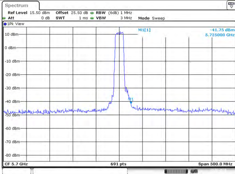
Plot on Configuration VHT20 / 5700 MHz / Peak / Port 1 (TX1)
