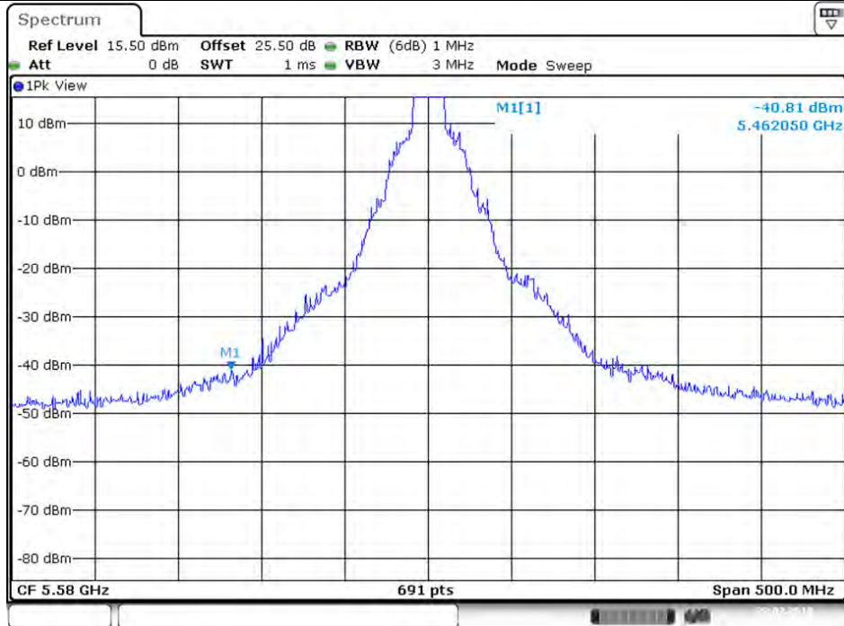
Plot on Configuration VHT20 / 5580 MHz / Peak / Port 1 (TX1)
