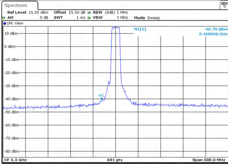
Plot on Configuration VHT20 / 5500 MHz / Peak / Port 2 (TX2)
