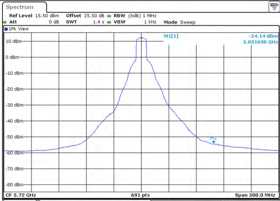
Plot on Configuration VHT20 / 5720 MHz / Average / Port 2 (TX2)
