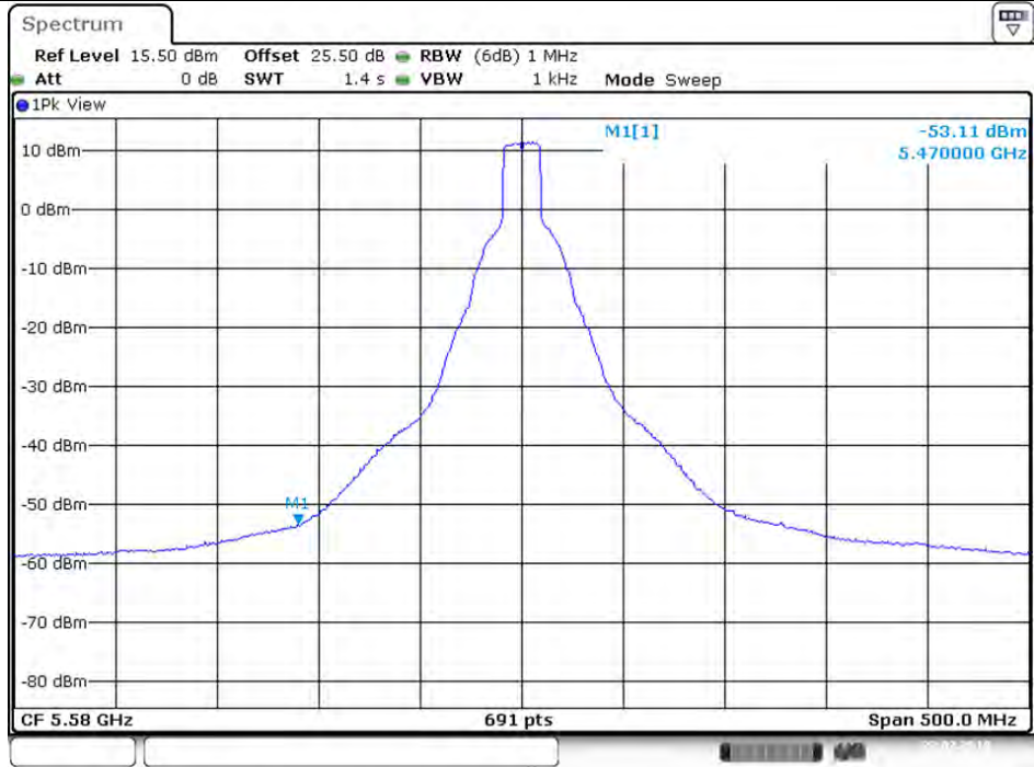
Plot on Configuration VHT20 / 5580 MHz / Average / Port 1 (TX1)
