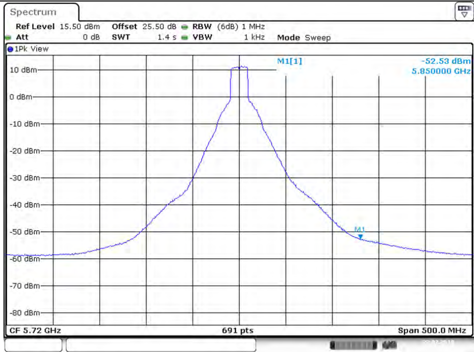
Plot on Configuration VHT20 / 5720 MHz / Average / Port 1 (TX1)
