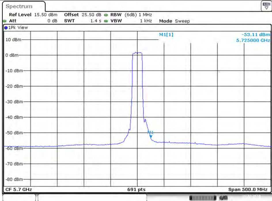
Plot on Configuration VHT20 / 5700 MHz / Average / Port 1 (TX1)
