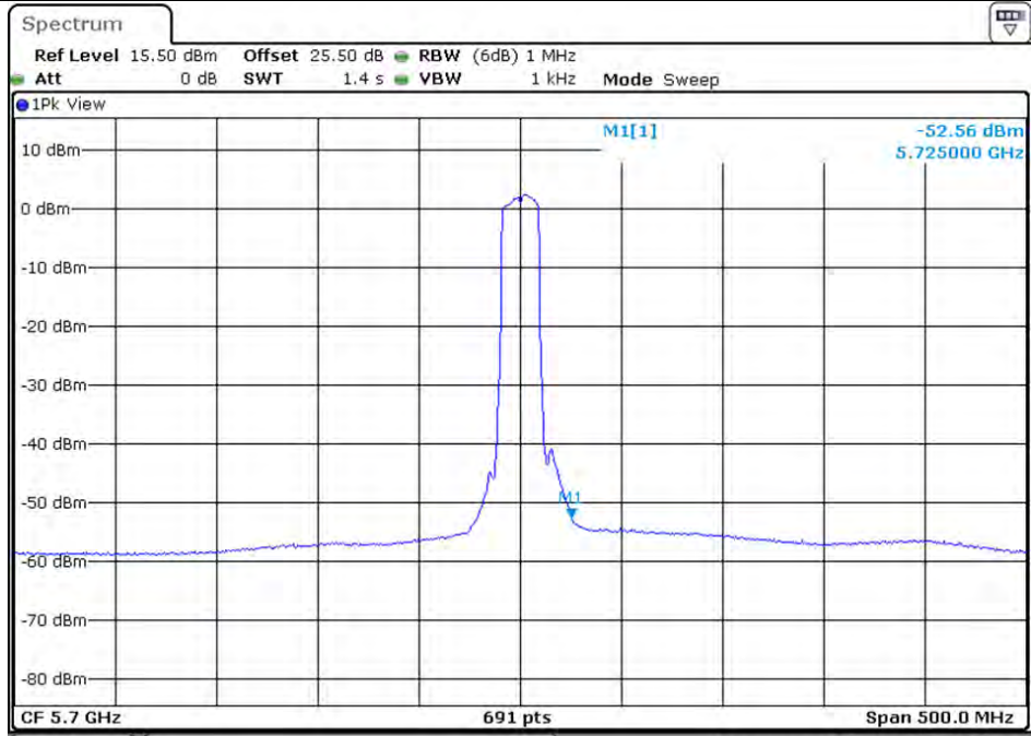
Plot on Configuration VHT20 / 5700 MHz / Average / Port 2 (TX2)
