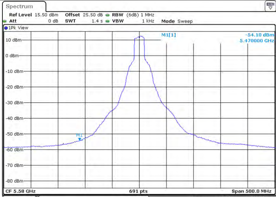
Plot on Configuration VHT20 / 5580 MHz / Average / Port 2 (TX2)
