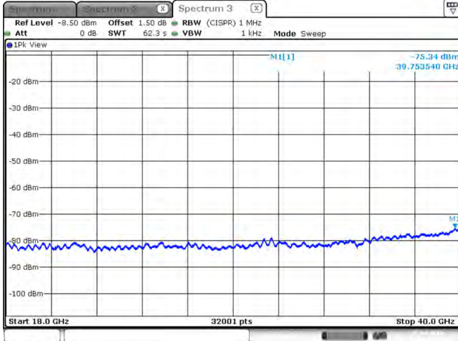
Plot on Configuration VHT80 / 5290 MHz / Average / Port 2 / 18GHz~40GHz
