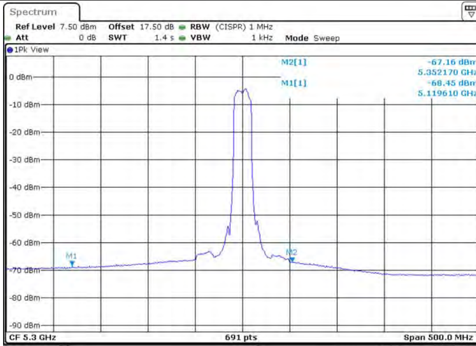
Plot on Configuration VHT20 / 5300 MHz / Average / Port 4
