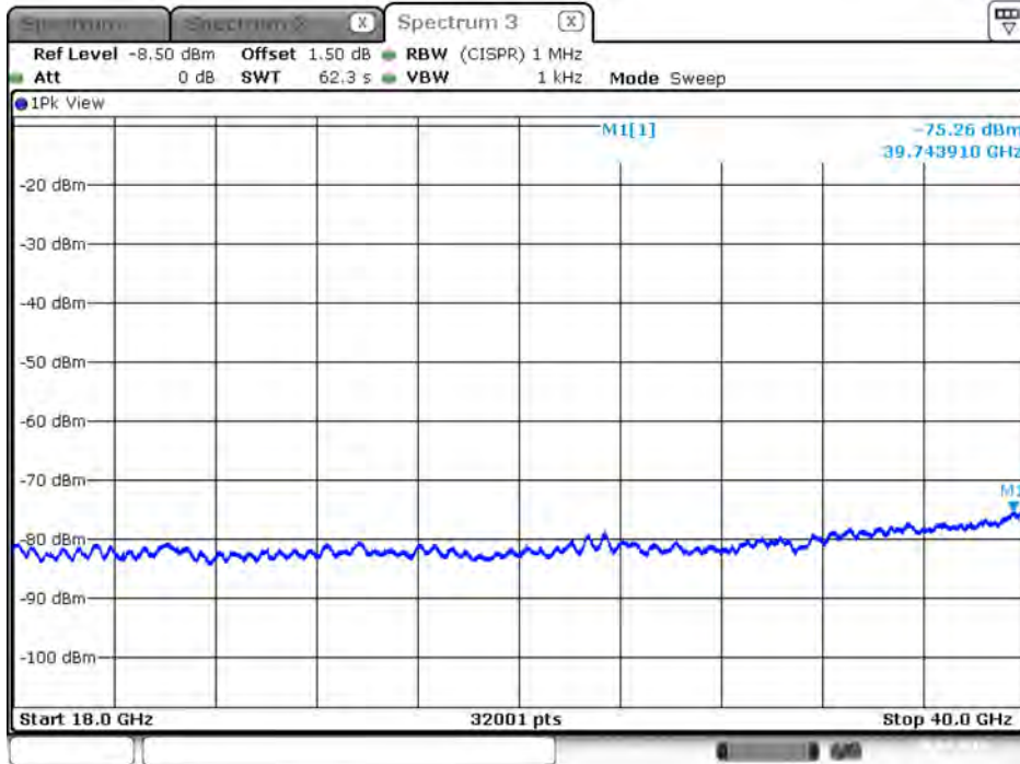
Plot on Configuration VHT80 / 5290 MHz / Average / Port 1 / 18GHz~40GHz
