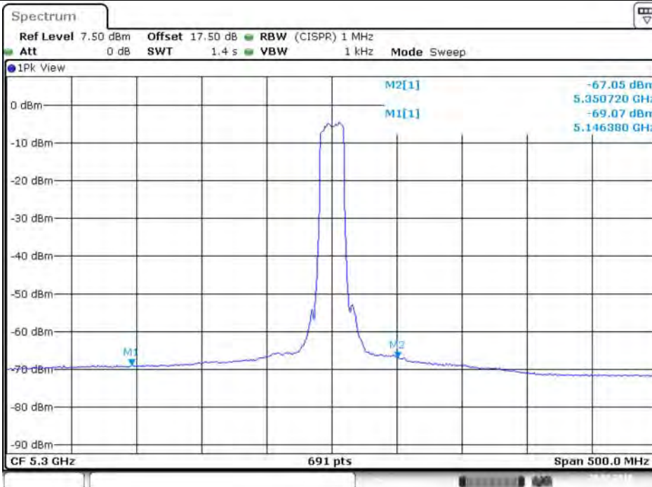
Plot on Configuration VHT20 / 5300 MHz / Average / Port 2
