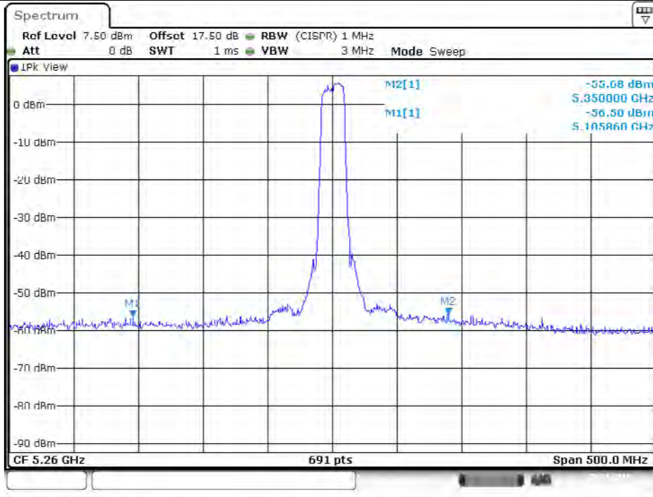
Plot on Configuration VHT20 / 5260 MHz / Peak / Port 3
