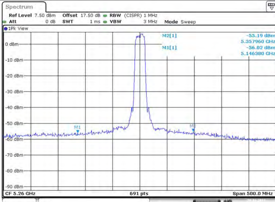
Plot on Configuration VHT20 / 5260 MHz / Peak / Port 4
