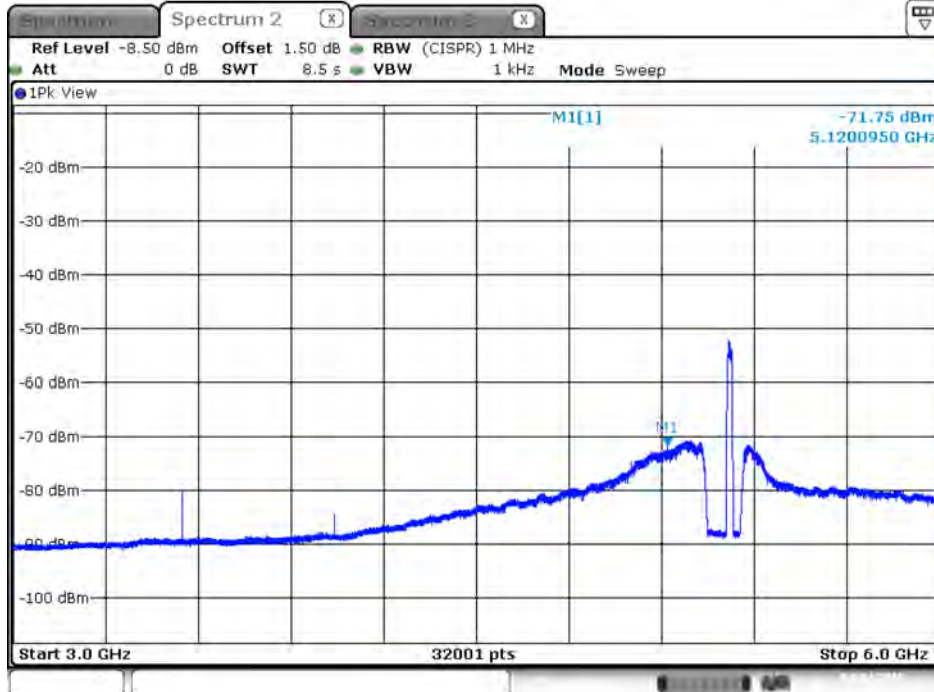
Plot on Configuration VHT20 / 5320 MHz / Average / Port 4 / 3GHz~6GHz
