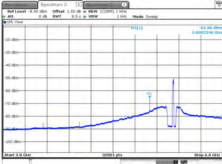
Plot on Configuration VHT20 / 5320 MHz / Average / Port 2 / 3GHz~6GHz
