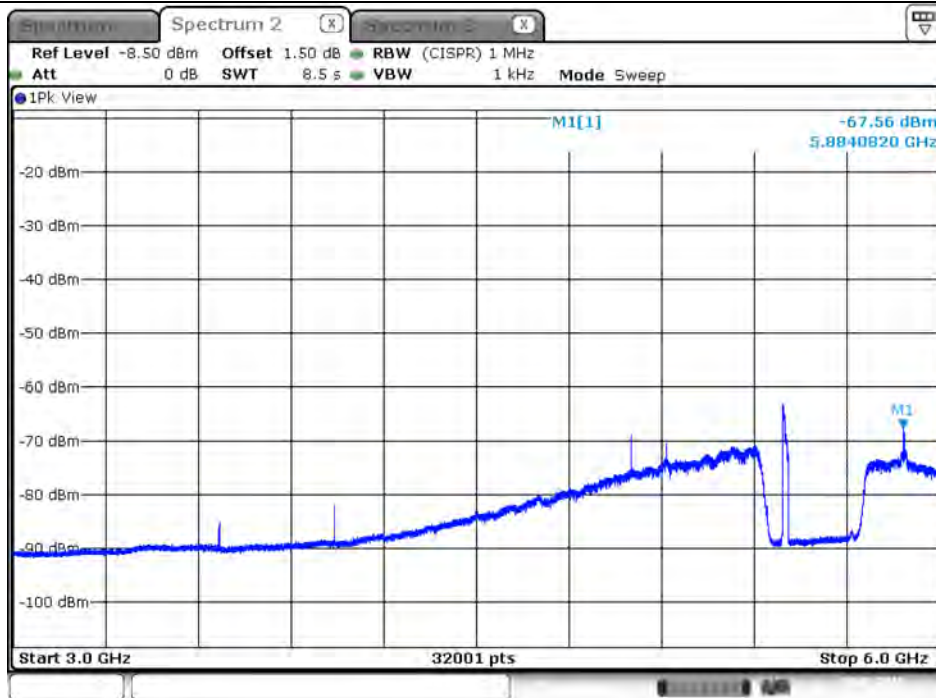
Plot on Configuration VHT20 / 5500 MHz / Average / Port 2 / 3GHz~6GHz
