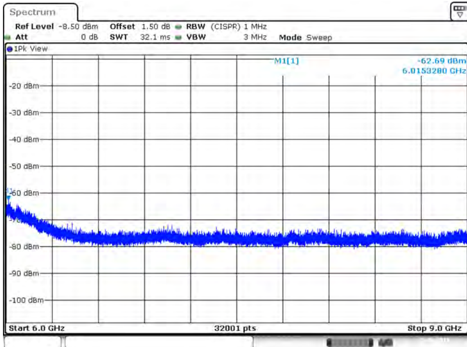
Plot on IEEE 802.11ac Nss1 MCS0 VHT80 / 5290 MHz / Peak / Port 1 / 6GHz~9GHz
