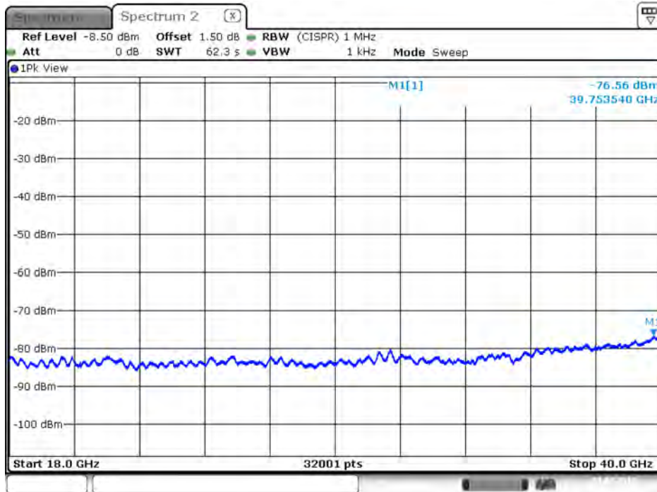
Plot on IEEE 802.11ac Nss1 MCS0 VHT20 / 5300 MHz / Average / Port 1 / 18GHz~40GHz
