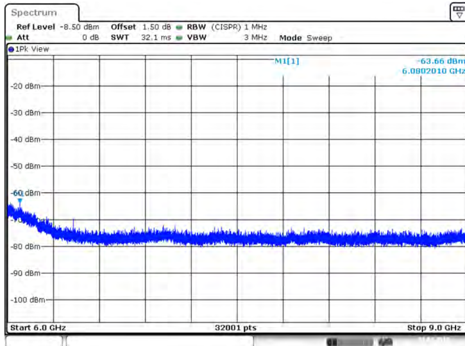
Plot on IEEE 802.11ac Nss1 MCS0 VHT20 / 5320 MHz / Peak / Port 2 / 6GHz~9GHz
