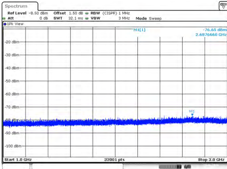
Plot on IEEE 802.11ac Nss1 MCS0 VHT80 / 5290 MHz / Peak / Port 2 / 1GHz~3GHz
