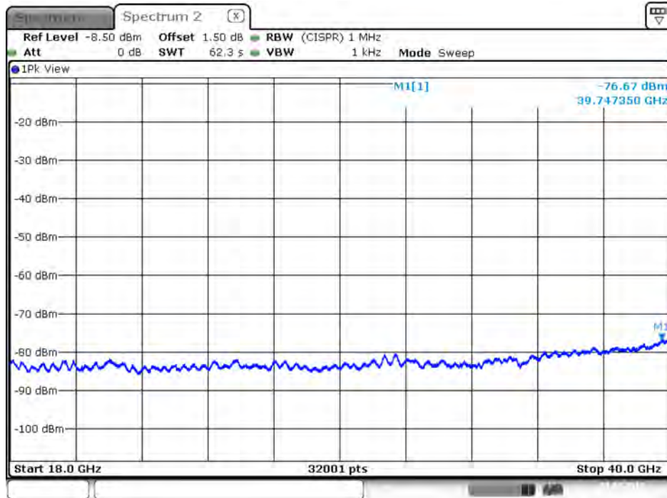
Plot on IEEE 802.11ac Nss1 MCS0 VHT20 / 5260 MHz / Average / Port 1 / 18GHz~40GHz
