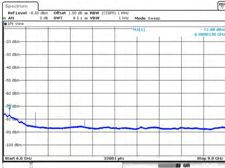
Plot on IEEE 802.11ac Nss1 MCS0 VHT20 / 5320 MHz / Average / Port 2 / 6GHz~9GHz
