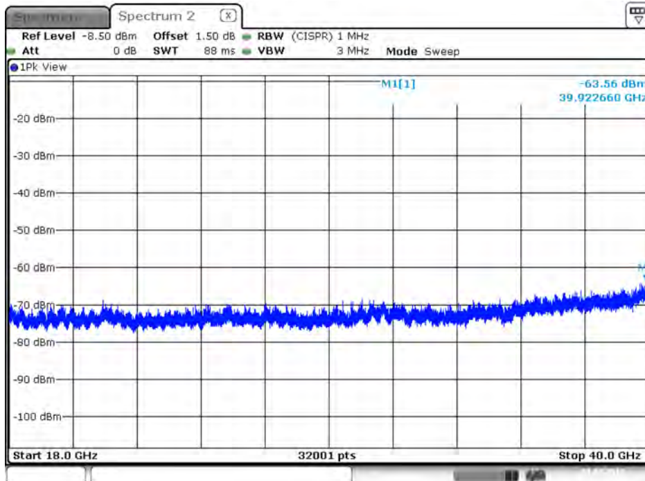
Plot on IEEE 802.11ac Nss1 MCS0 VHT20 / 5300 MHz / Peak / Port 1 / 18GHz~40GHz
