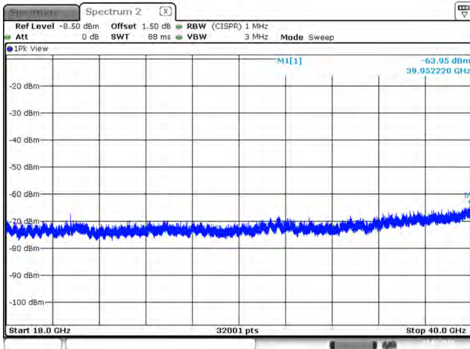
Plot on IEEE 802.11ac Nss1 MCS0 VHT20 / 5260 MHz / Peak / Port 2 / 18GHz~40GHz
