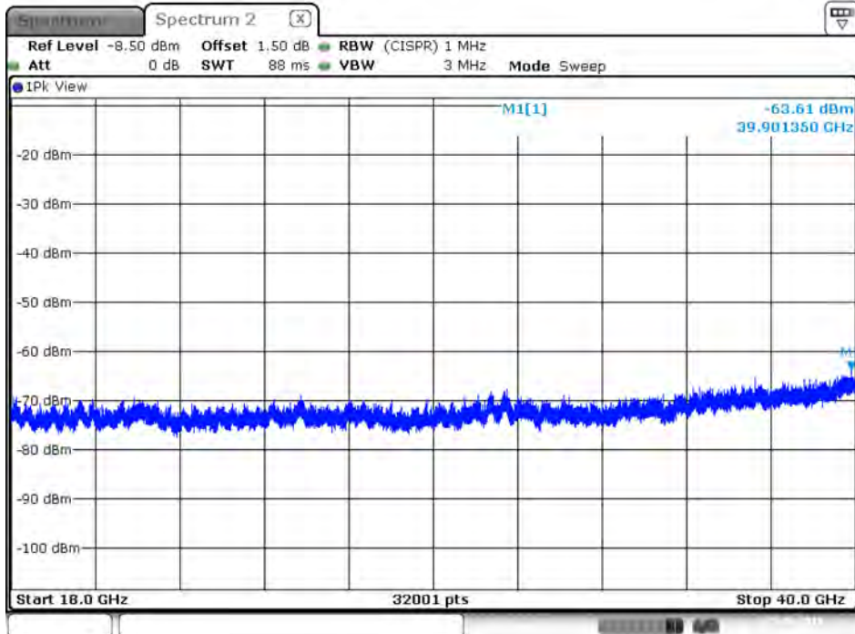
Plot on IEEE 802.11ac Nss1 MCS0 VHT80 / 5290 MHz / Peak / Port 1 / 18GHz~40GHz
