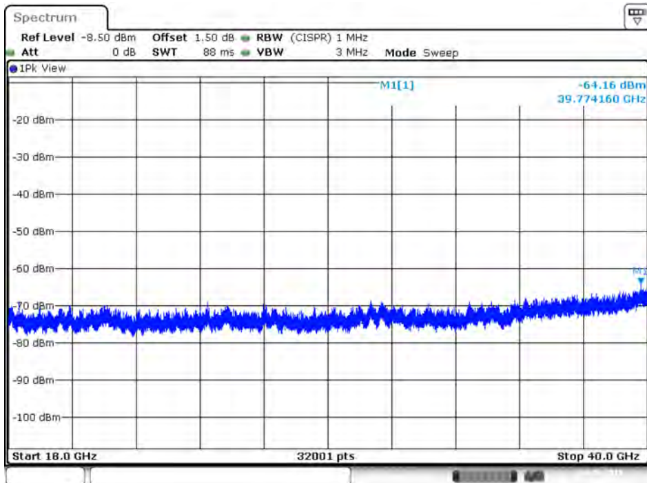
Plot on IEEE 802.11ac Nss1 MCS0 VHT80 / 5610 MHz / Peak / Port 2 / 18GHz~40GHz
