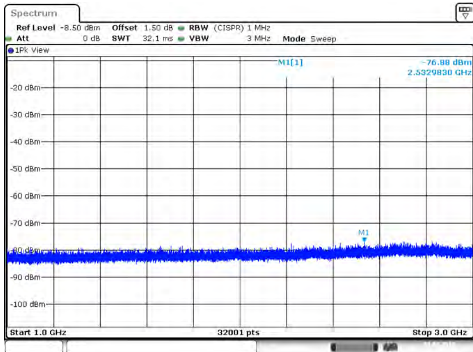
Plot on IEEE 802.11ac Nss1 MCS0 VHT20 / 5260 MHz / Peak / Port 1 / 1GHz~3GHz
