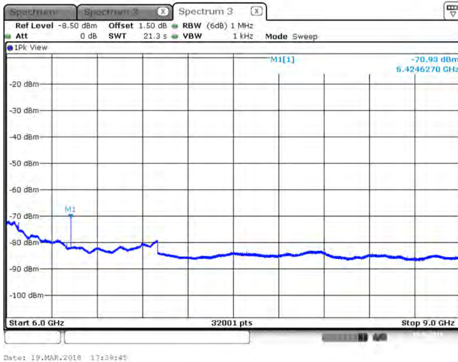
Plot on IEEE 802.11ac Nss1 MCS0 VHT80 / 5690 MHz / Peak / Port 2 / 6GHz~9GHz
