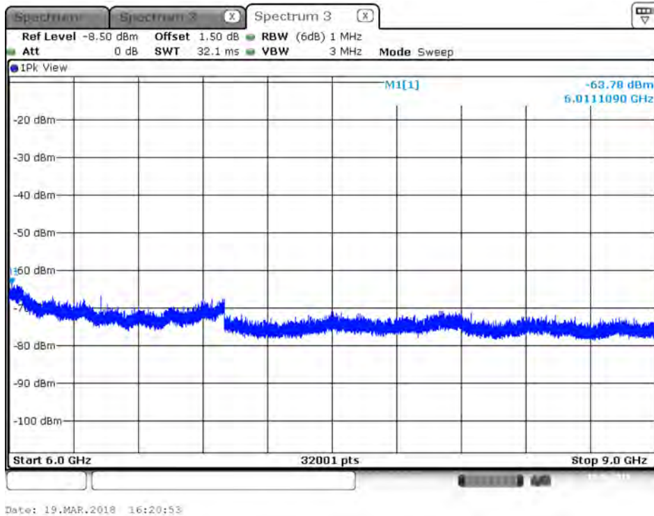
Plot on IEEE 802.11ac Nss1 MCS0 VHT80 / 5610 MHz / Peak / Port 2 / 6GHz~9GHz
