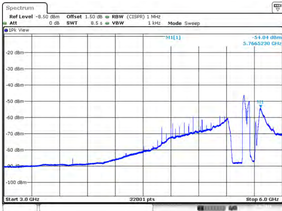
Plot on IEEE 802.11ac Nss1 MCS0 VHT80 / 5610 MHz / Average / Port 1 / 3GHz~6GHz
