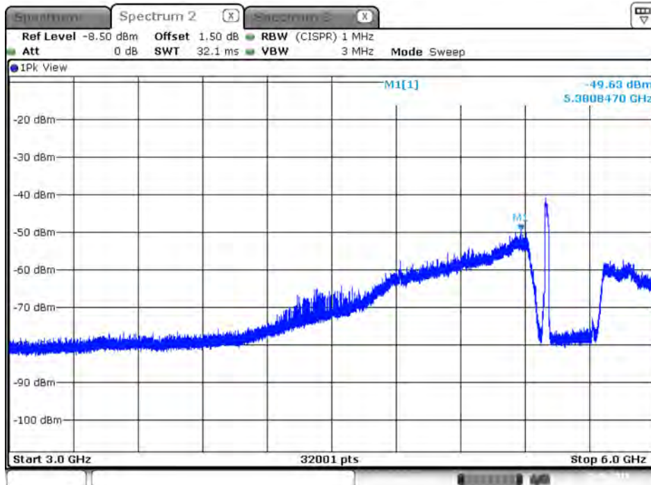
Plot on IEEE 802.11ac Nss1 MCS0 VHT20 / 5500 MHz / Peak / Port 1 / 3GHz~6GHz
