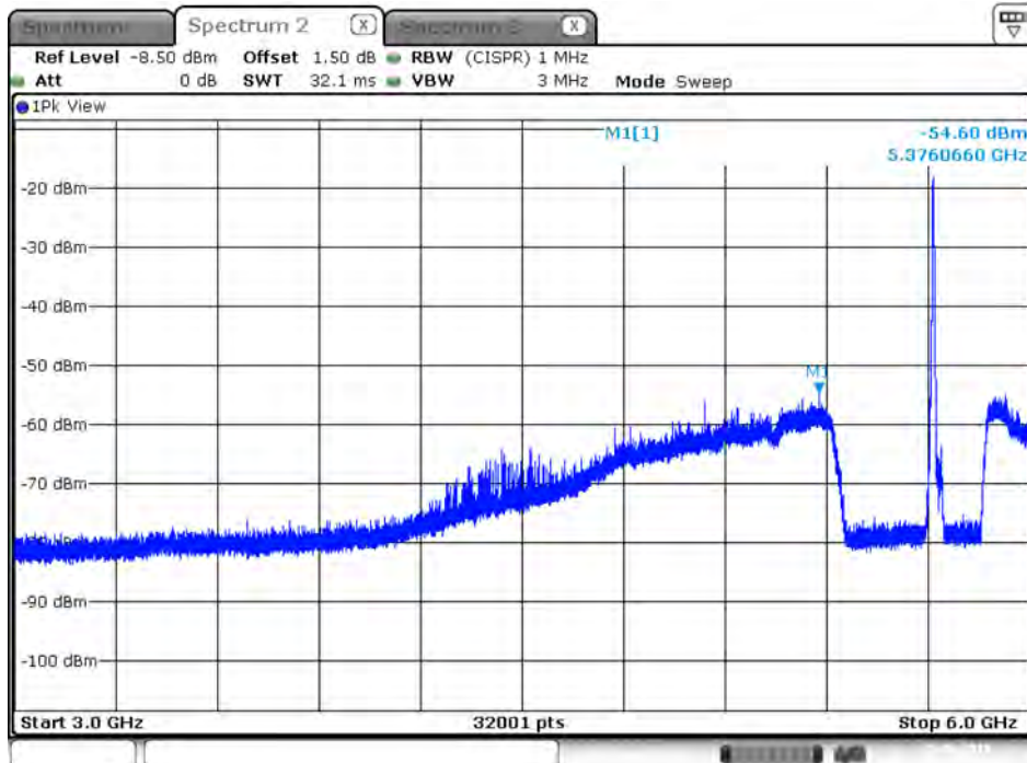
Plot on IEEE 802.11ac Nss1 MCS0 VHT20 / 5720 MHz / Peak / Port 1 / 3GHz~6GHz
