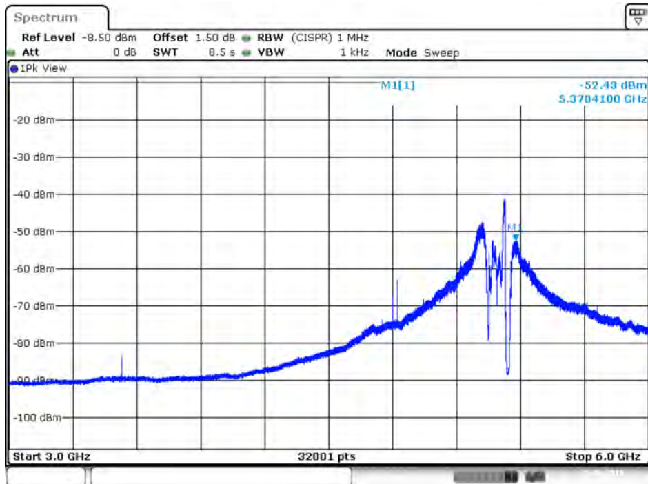
Plot on IEEE 802.11ac Nss1 MCS0 VHT80 / 5290 MHz / Average / Port 2 / 3GHz~6GHz
