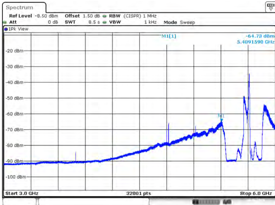
Plot on IEEE 802.11ac Nss1 MCS0 VHT80 / 5690 MHz / Average / Port 1 / 3GHz~6GHz
