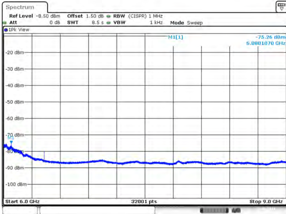
Plot on IEEE 802.11ac Nss1 MCS0 VHT80 / 5290 MHz / Average / Port 1 / 6GHz~9GHz
