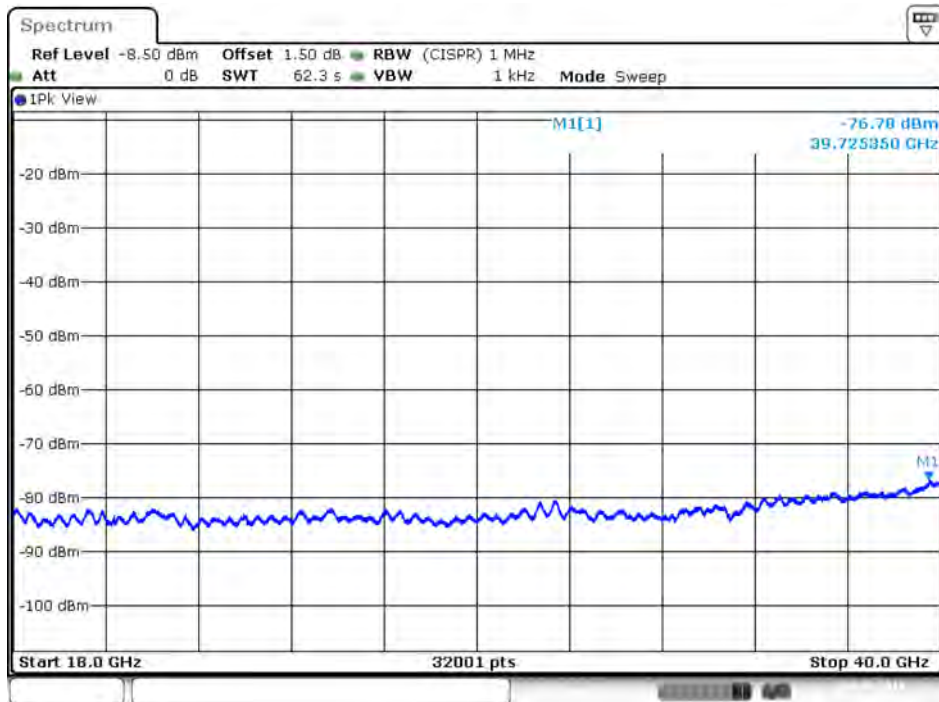
Plot on IEEE 802.11ac Nss1 MCS0 VHT20 / 5580 MHz / Average / Port 2 / 18GHz~40GHz
