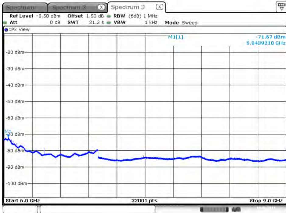
Plot on IEEE 802.11ac Nss1 MCS0 VHT80 / 5610 MHz / Average / Port 1 / 6GHz~9GHz
