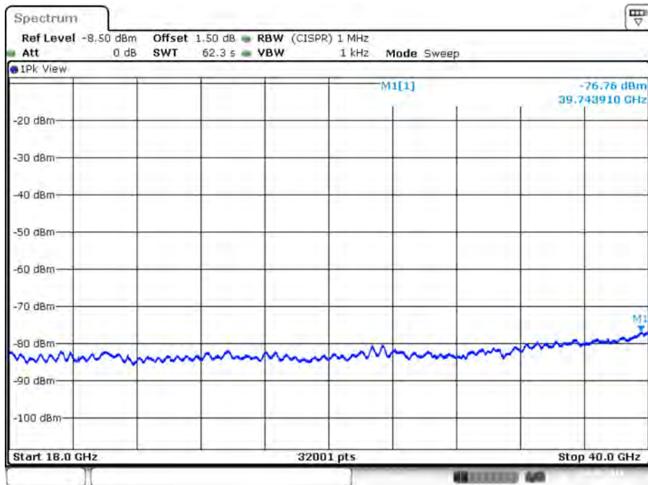
Plot on IEEE 802.11ac Nss1 MCS0 VHT80 / 5610 MHz / Average / Port 1 / 18GHz~40GHz
