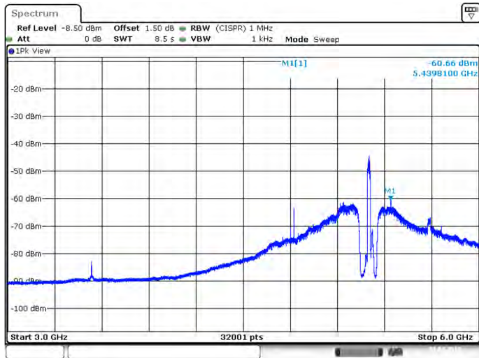
Plot on IEEE 802.11ac Nss1 MCS0 VHT20 / 5300 MHz / Average / Port 2 / 3GHz~6GHz
