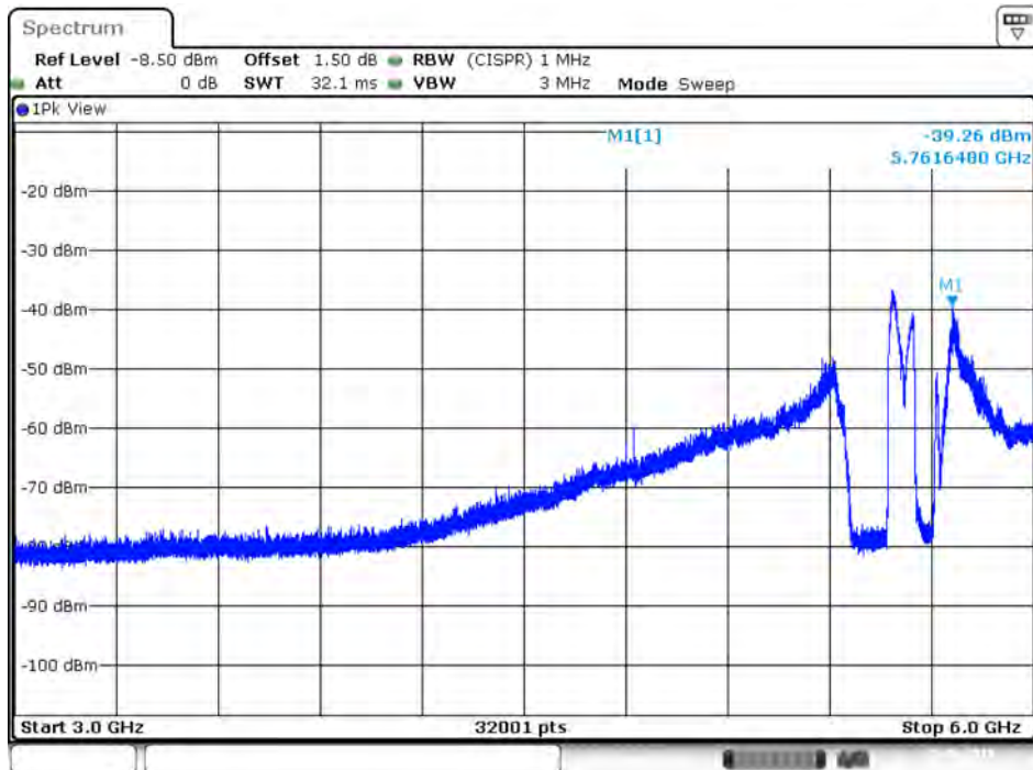
Plot on IEEE 802.11ac Nss1 MCS0 VHT80 / 5610 MHz / Peak / Port 2 / 3GHz~6GHz
