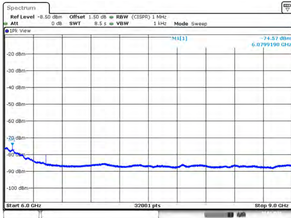
Plot on IEEE 802.11ac Nss1 MCS0 VHT20 / 5320 MHz / Average / Port 1 / 6GHz~9GHz
