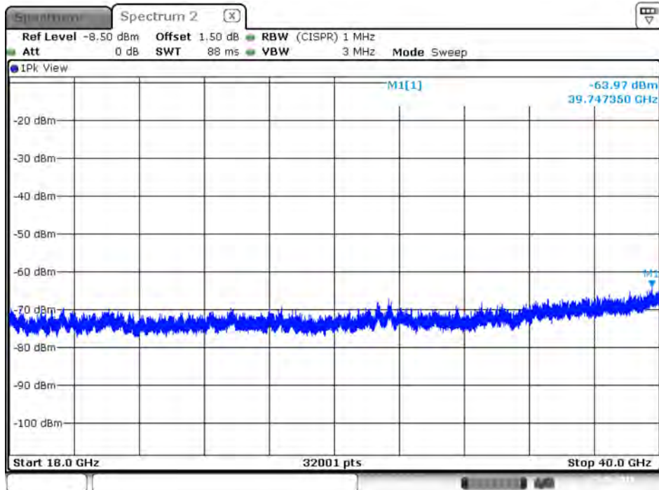
Plot on IEEE 802.11ac Nss1 MCS0 VHT80 / 5290 MHz / Peak / Port 2 / 18GHz~40GHz
