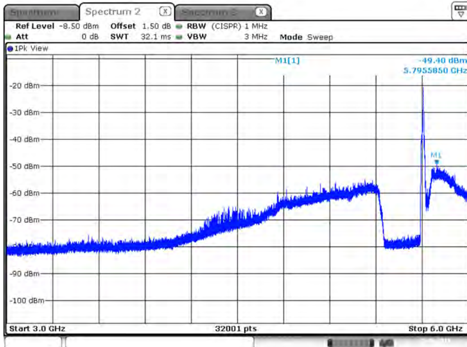
Plot on IEEE 802.11ac Nss1 MCS0 VHT20 / 5700 MHz / Peak / Port 1 / 3GHz~6GHz
