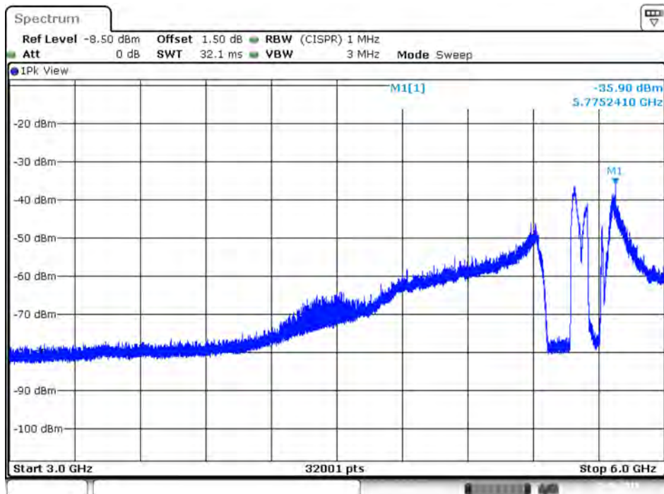
Plot on IEEE 802.11ac Nss1 MCS0 VHT80 / 5610 MHz / Peak / Port 1 / 3GHz~6GHz
