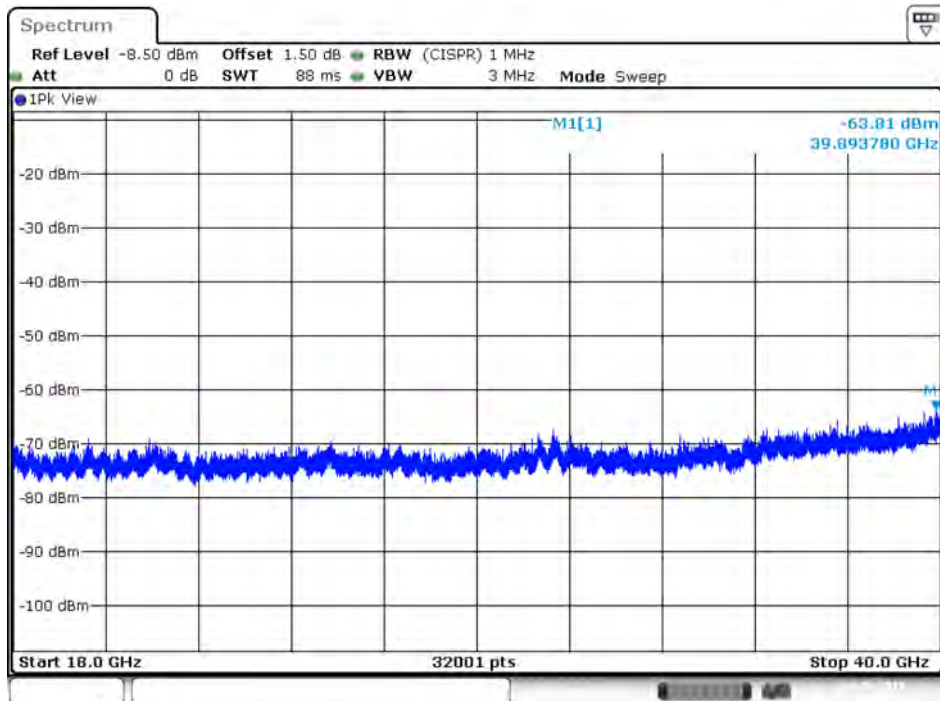
Plot on IEEE 802.11ac Nss1 MCS0 VHT80 / 5530 MHz / Peak / Port 1 / 18GHz~40GHz
