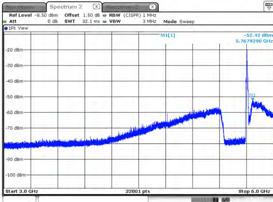
Plot on IEEE 802.11ac Nss1 MCS0 VHT20 / 5700 MHz / Peak / Port 2 / 3GHz~6GHz
