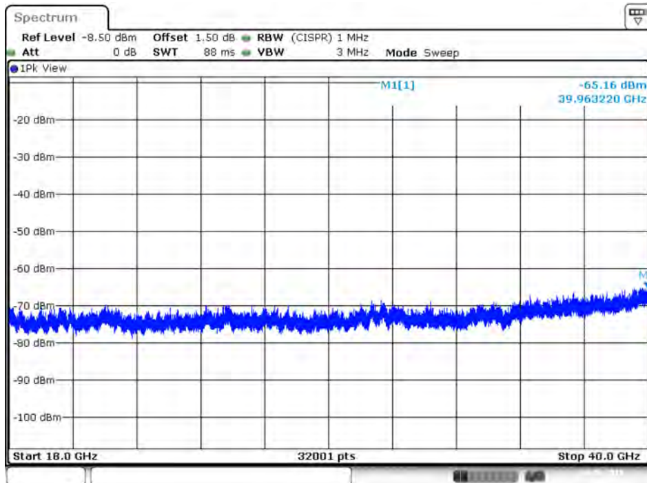
Plot on IEEE 802.11ac Nss1 MCS0 VHT20 / 5580 MHz / Peak / Port 2 / 18GHz~40GHz
