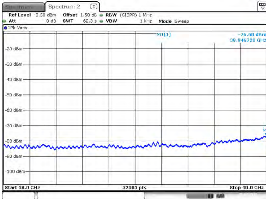
Plot on IEEE 802.11ac Nss1 MCS0 VHT20 / 5260 MHz / Average / Port 2 / 18GHz~40GHz
