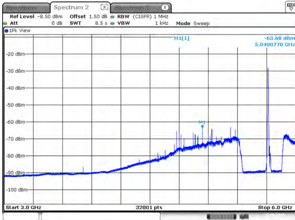
Plot on IEEE 802.11ac Nss1 MCS0 VHT20 / 5720 MHz / Average / Port 1 / 3GHz~6GHz
