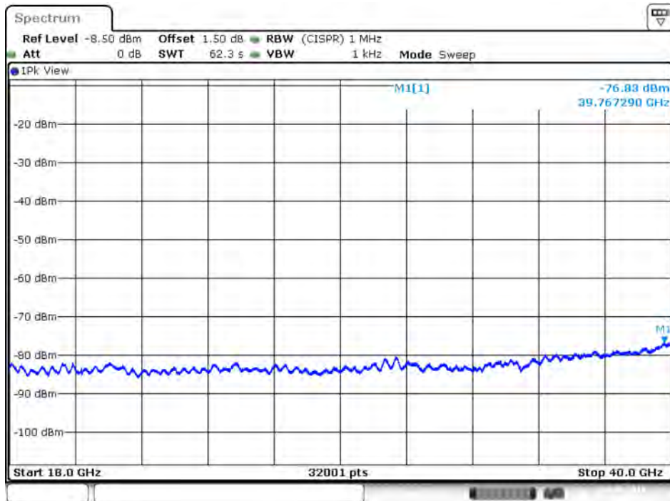
Plot on IEEE 802.11ac Nss1 MCS0 VHT20 / 5720 MHz / Average / Port 2 / 18GHz~40GHz
