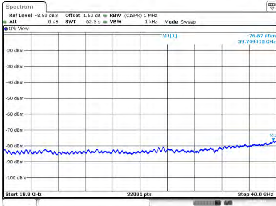
Plot on IEEE 802.11ac Nss1 MCS0 VHT20 / 5580 MHz / Average / Port 1 / 18GHz~40GHz
