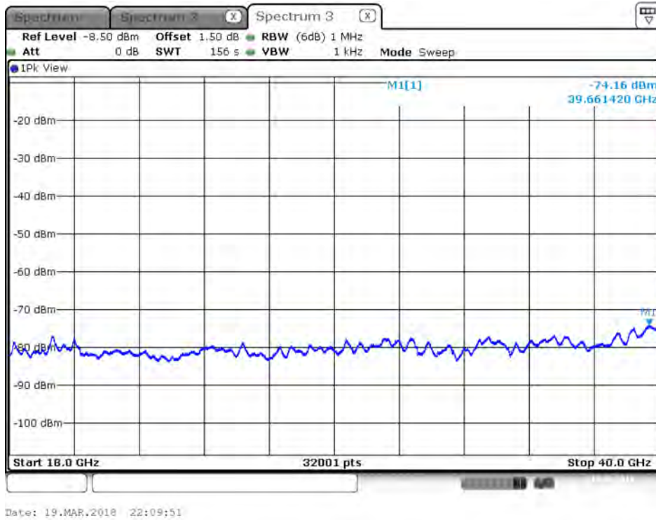
Plot on IEEE 802.11ac Nss1 MCS0 VHT80 / 5690 MHz / Peak / Port 1 / 18GHz~40GHz
