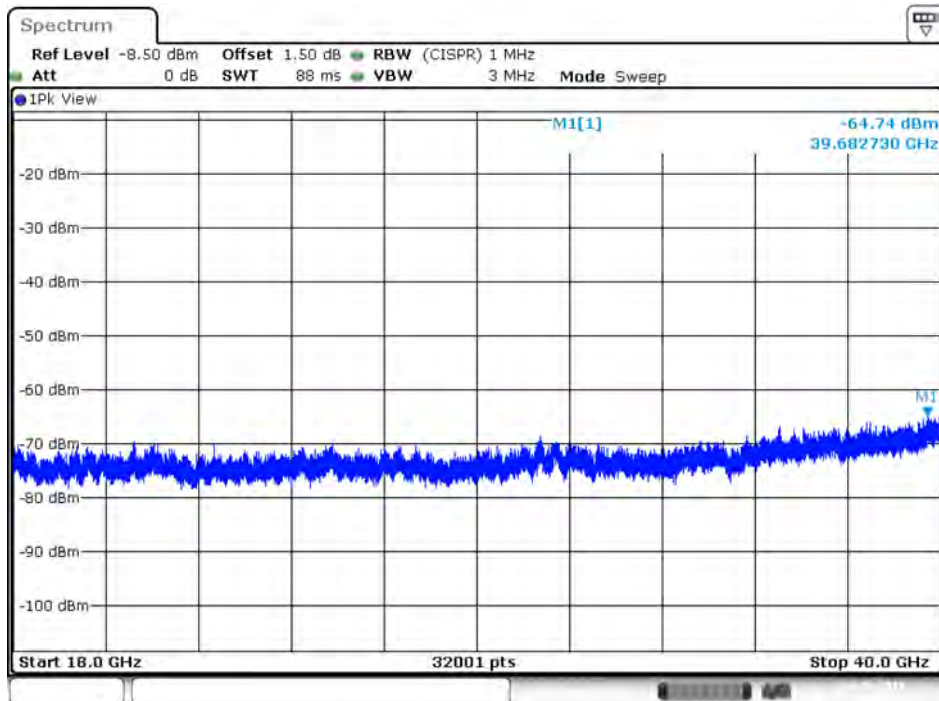
Plot on IEEE 802.11ac Nss1 MCS0 VHT20 / 5720 MHz / Peak / Port 2 / 18GHz~40GHz
