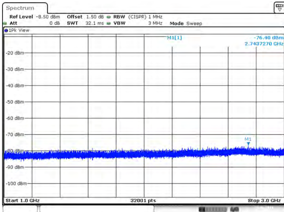
Plot on IEEE 802.11ac Nss1 MCS0 VHT80 / 5290 MHz / Peak / Port 1 / 1GHz~3GHz
