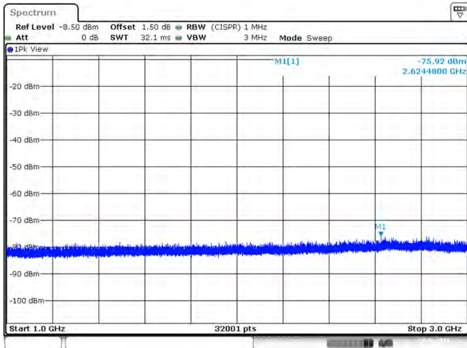
Plot on IEEE 802.11ac Nss1 MCS0 VHT80 / 5690 MHz / Peak / Port 2 / 1GHz~3GHz
