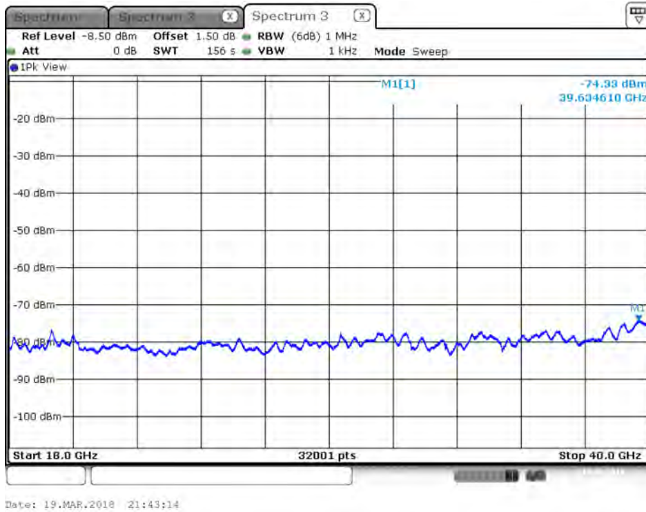
Plot on IEEE 802.11ac Nss1 MCS0 VHT80 / 5530 MHz / Peak / Port 2 / 18GHz~40GHz
