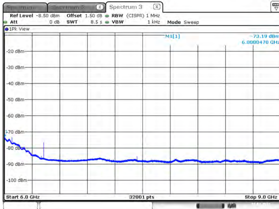
Plot on IEEE 802.11ac Nss1 MCS0 VHT20 / 5580 MHz / Average / Port 2 / 6GHz~9GHz
