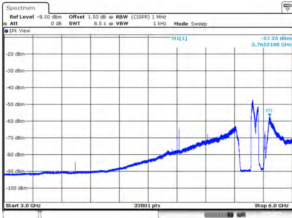
Plot on IEEE 802.11ac Nss1 MCS0 VHT80 / 5610 MHz / Average / Port 2 / 3GHz~6GHz
