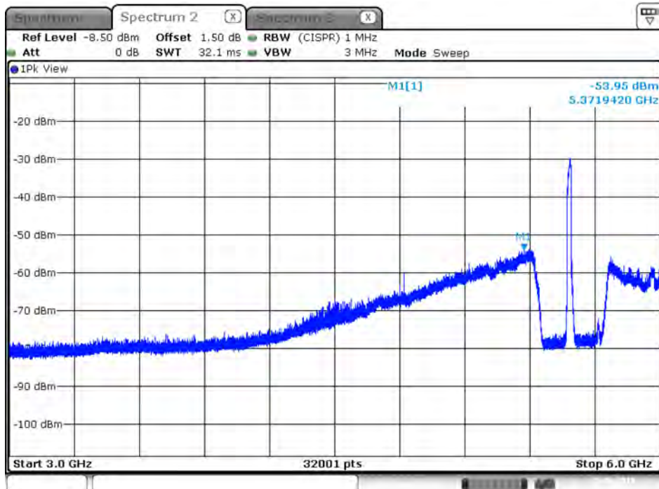
Plot on IEEE 802.11ac Nss1 MCS0 VHT20 / 5580 MHz / Peak / Port 2 / 3GHz~6GHz
