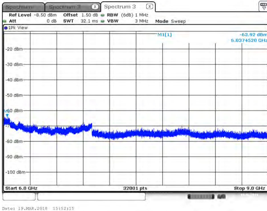
Plot on IEEE 802.11ac Nss1 MCS0 VHT80 / 5530 MHz / Peak / Port 1 / 6GHz~9GHz
