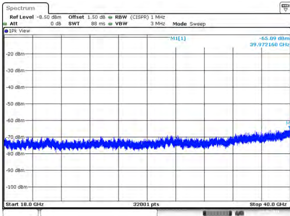
Plot on IEEE 802.11ac Nss1 MCS0 VHT80 / 5610 MHz / Peak / Port 1 / 18GHz~40GHz
