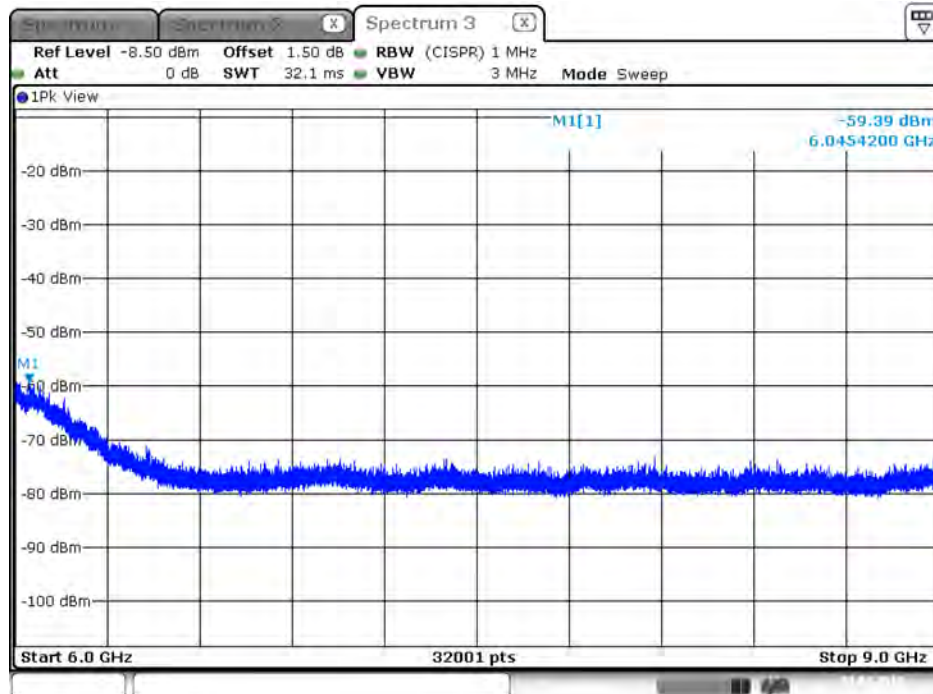
Plot on IEEE 802.11ac Nss1 MCS0 VHT20 / 5700 MHz / Peak / Port 1 / 6GHz~9GHz
