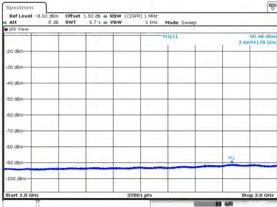
Plot on IEEE 802.11ac Nss1 MCS0 VHT80 / 5690 MHz / Average / Port 2 / 1GHz~3GHz
