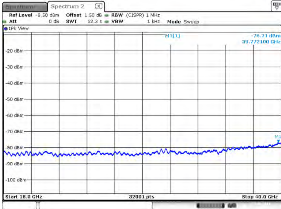
Plot on IEEE 802.11ac Nss1 MCS0 VHT80 / 5290 MHz / Average / Port 1 / 18GHz~40GHz
