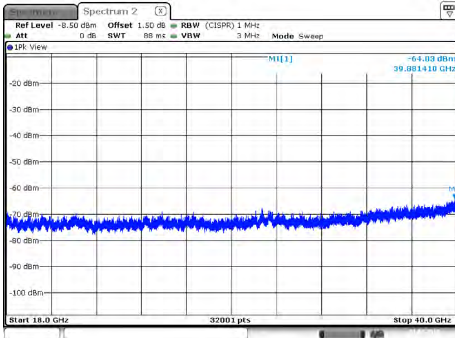
Plot on IEEE 802.11ac Nss1 MCS0 VHT20 / 5320 MHz / Peak / Port 1 / 18GHz~40GHz
