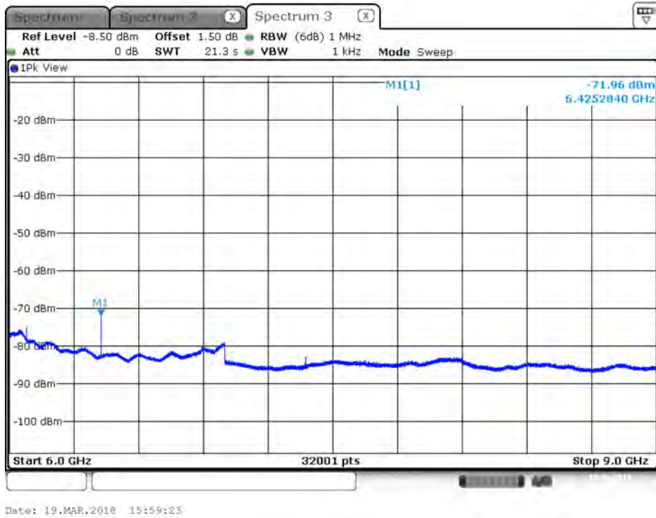
Plot on IEEE 802.11ac Nss1 MCS0 VHT80 / 5530 MHz / Peak / Port 2 / 6GHz~9GHz
