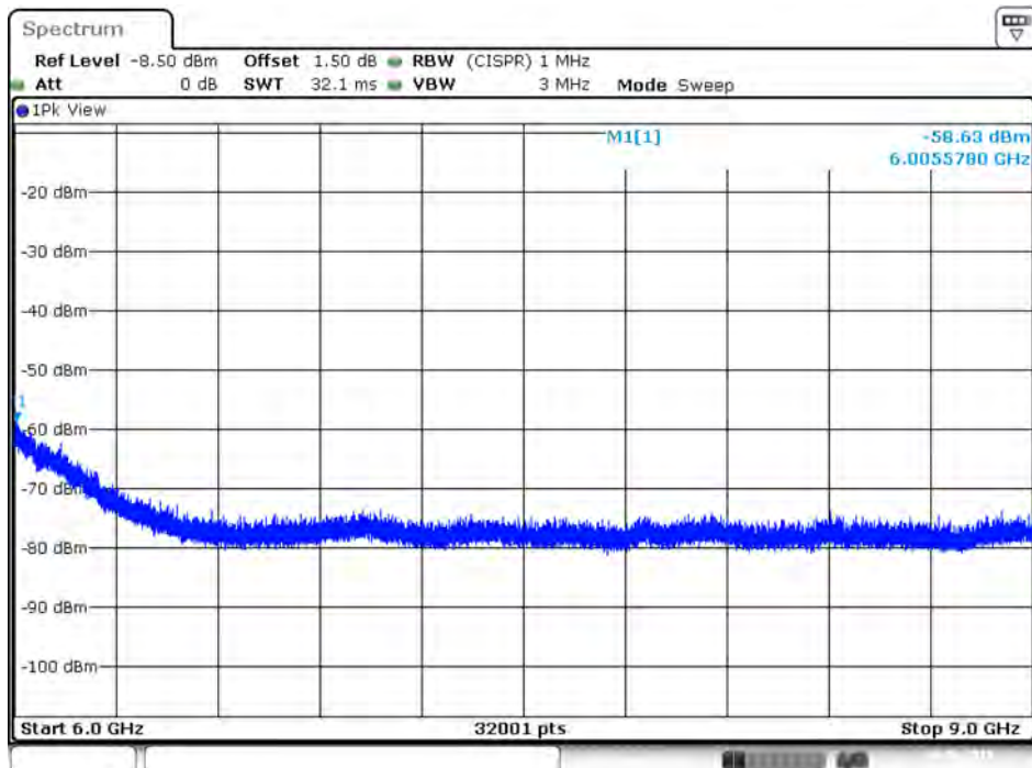
Plot on IEEE 802.11ac Nss1 MCS0 VHT80 / 5610 MHz / Peak / Port 1 / 6GHz~9GHz
