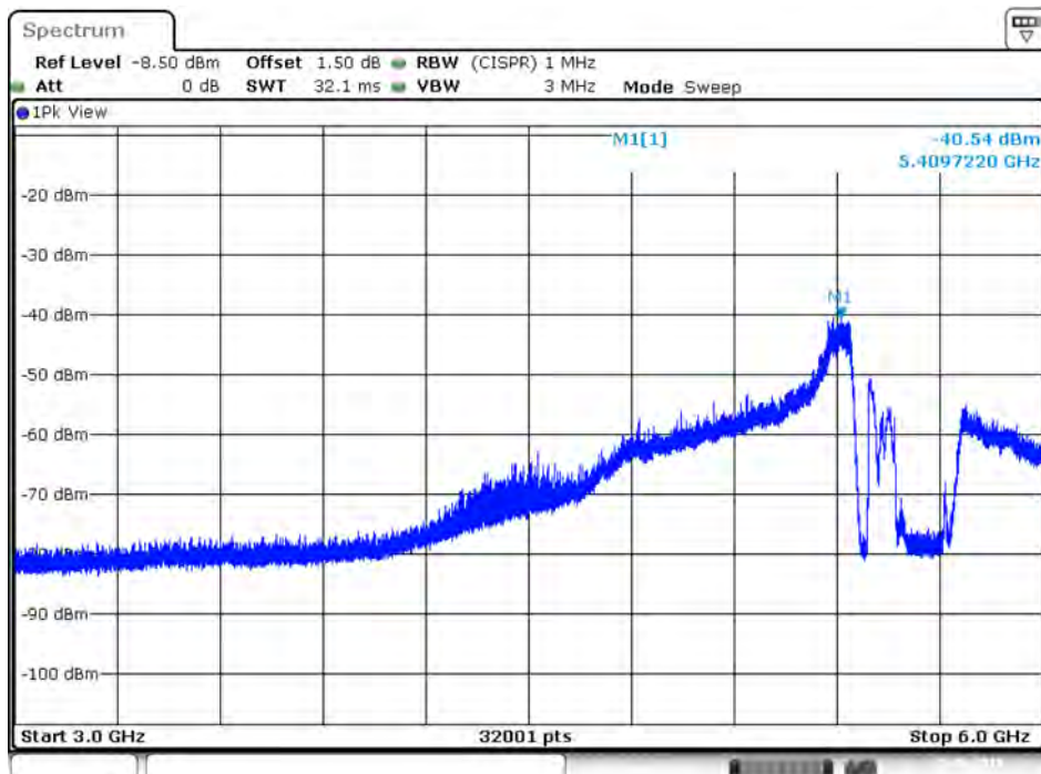
Plot on IEEE 802.11ac Nss1 MCS0 VHT80 / 5530 MHz / Peak / Port 1 / 3GHz~6GHz
