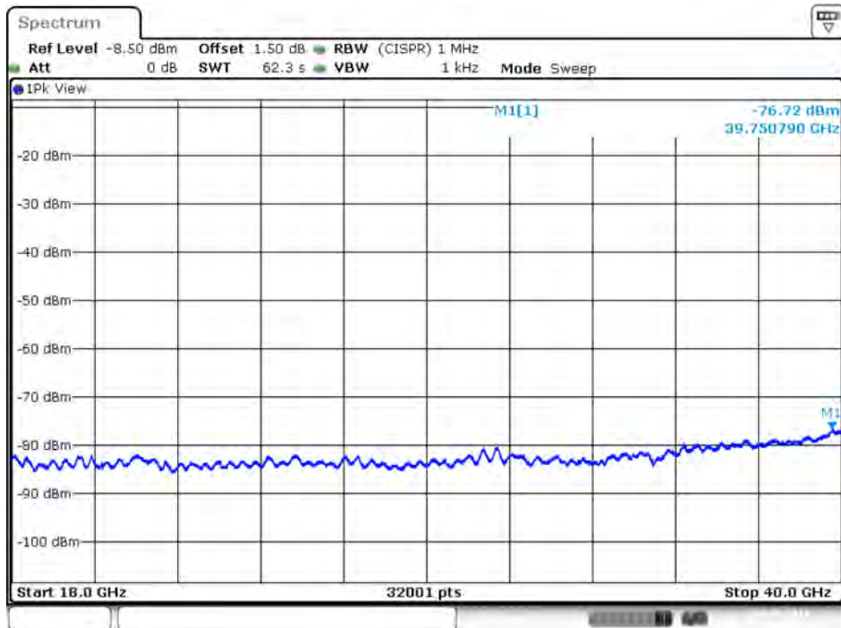
Plot on IEEE 802.11ac Nss1 MCS0 VHT20 / 5500 MHz / Average / Port 1 / 18GHz~40GHz
