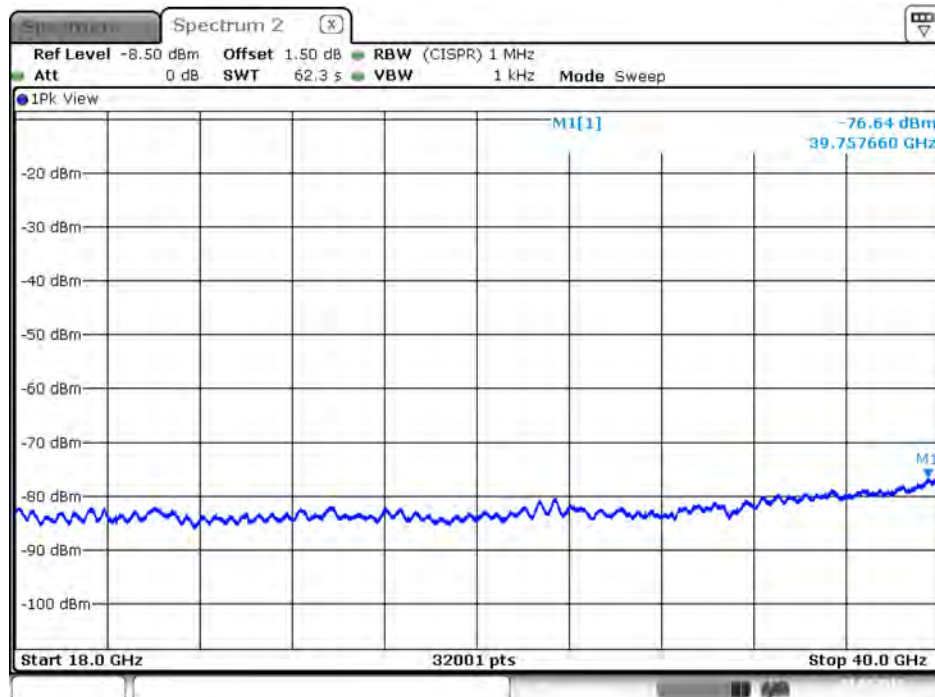
Plot on IEEE 802.11ac Nss1 MCS0 VHT20 / 5320 MHz / Average / Port 2 / 18GHz~40GHz
