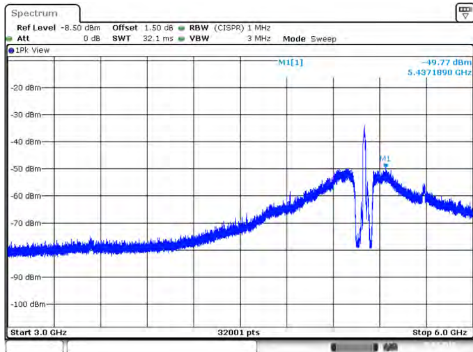
Plot on IEEE 802.11ac Nss1 MCS0 VHT20 / 5300 MHz / Peak / Port 2 / 3GHz~6GHz
