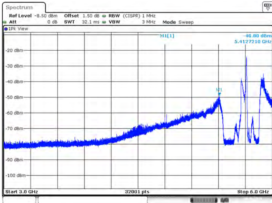
Plot on IEEE 802.11ac Nss1 MCS0 VHT80 / 5690 MHz / Peak / Port 1 / 3GHz~6GHz
