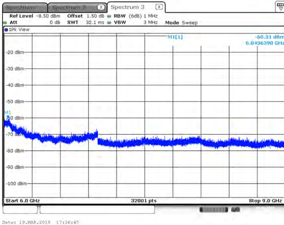
Plot on IEEE 802.11ac Nss1 MCS0 VHT80 / 5690 MHz / Peak / Port 1 / 6GHz~9GHz
