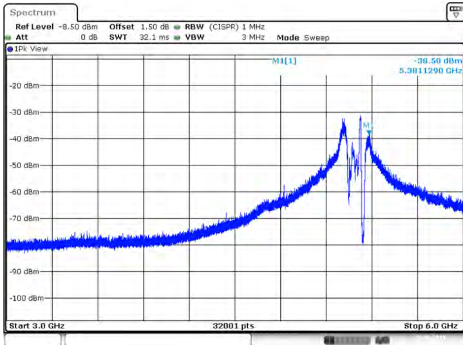
Plot on IEEE 802.11ac Nss1 MCS0 VHT80 / 5290 MHz / Peak / Port 2 / 3GHz~6GHz
