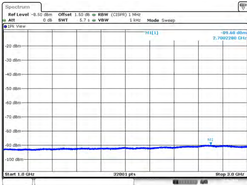
Plot on IEEE 802.11ac Nss1 MCS0 VHT80 / 5290 MHz / Average / Port 1 / 1GHz~3GHz
