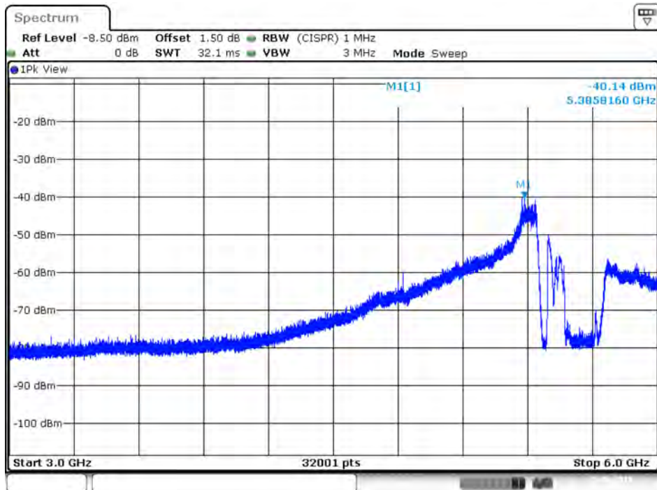
Plot on IEEE 802.11ac Nss1 MCS0 VHT80 / 5530 MHz / Peak / Port 2 / 3GHz~6GHz
