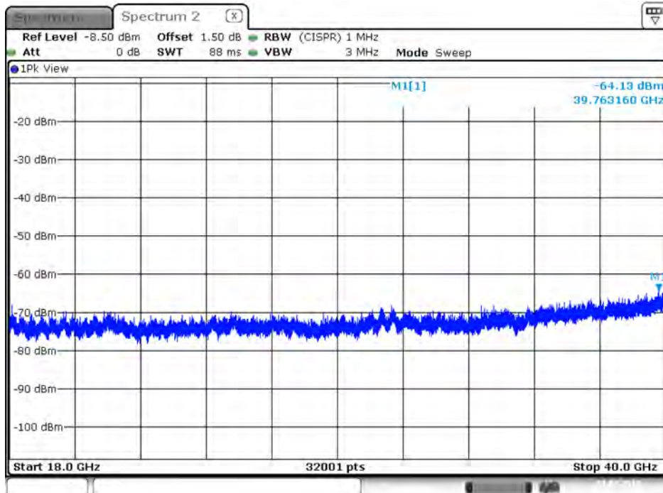
Plot on IEEE 802.11ac Nss1 MCS0 VHT20 / 5300 MHz / Peak / Port 2 / 18GHz~40GHz
