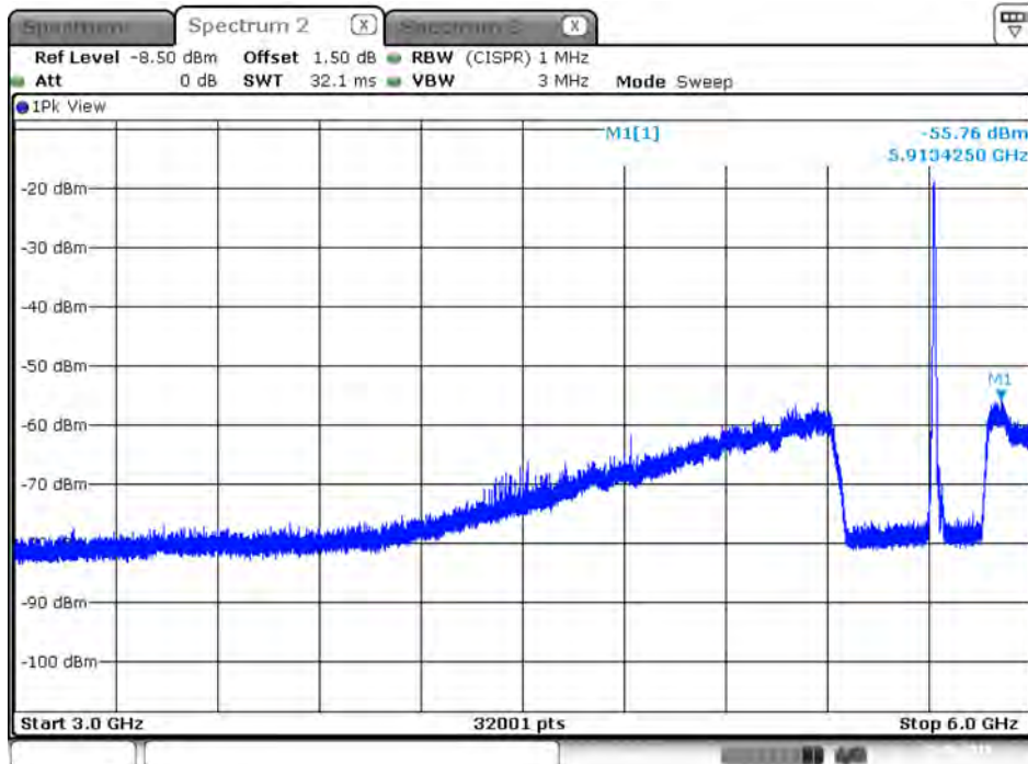
Plot on IEEE 802.11ac Nss1 MCS0 VHT20 / 5720 MHz / Peak / Port 2 / 3GHz~6GHz
