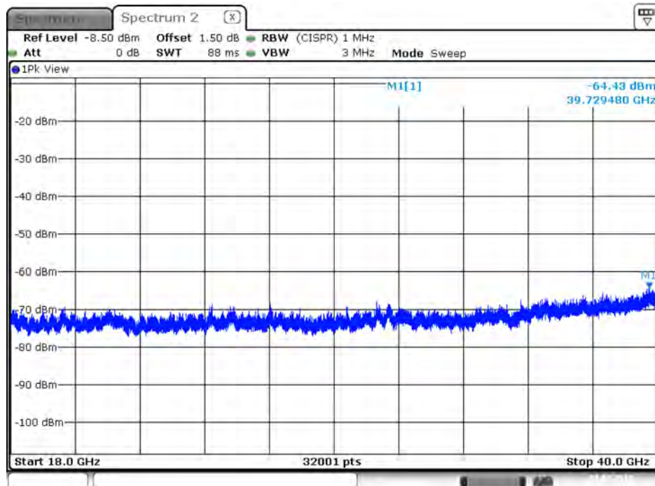
Plot on IEEE 802.11ac Nss1 MCS0 VHT20 / 5320 MHz / Peak / Port 2 / 18GHz~40GHz
