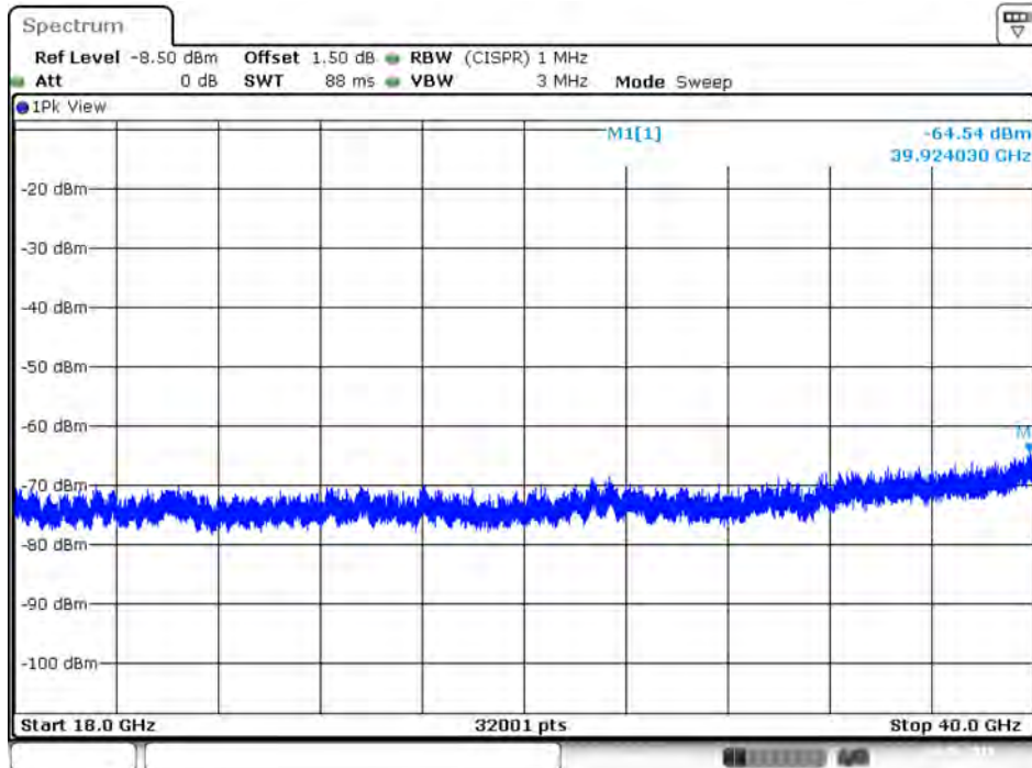
Plot on IEEE 802.11ac Nss1 MCS0 VHT20 / 5580 MHz / Peak / Port 1 / 18GHz~40GHz
