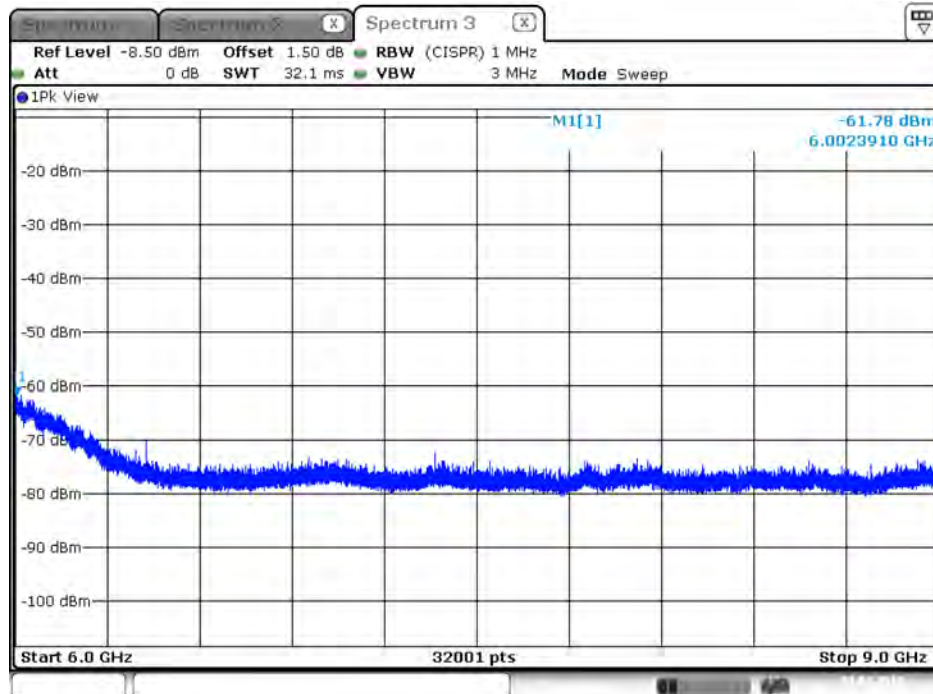
Plot on IEEE 802.11ac Nss1 MCS0 VHT20 / 5580 MHz / Peak / Port 2 / 6GHz~9GHz
