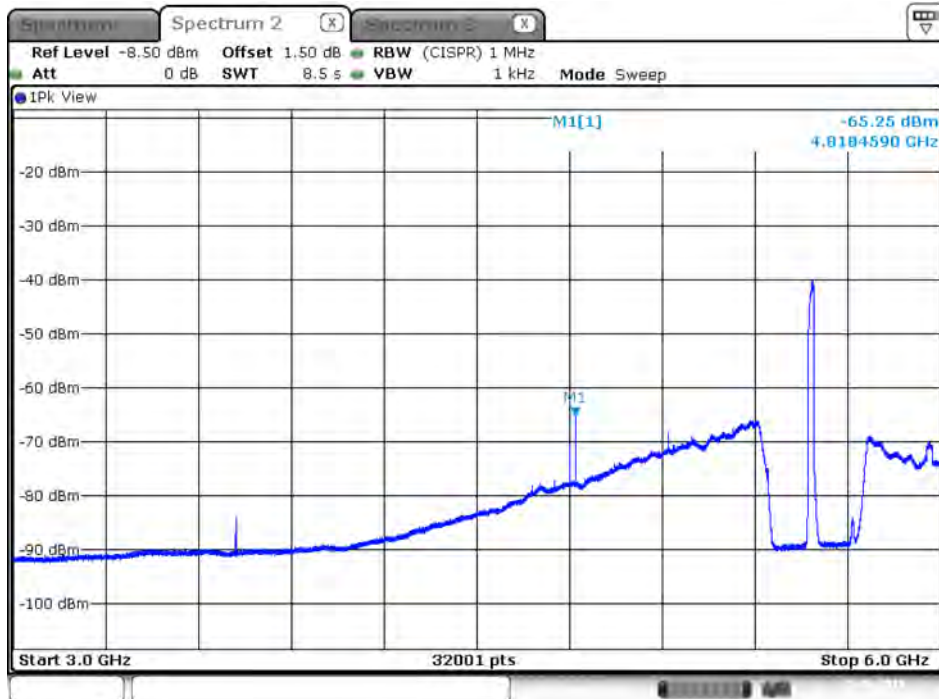
Plot on IEEE 802.11ac Nss1 MCS0 VHT20 / 5580 MHz / Average / Port 2 / 3GHz~6GHz
