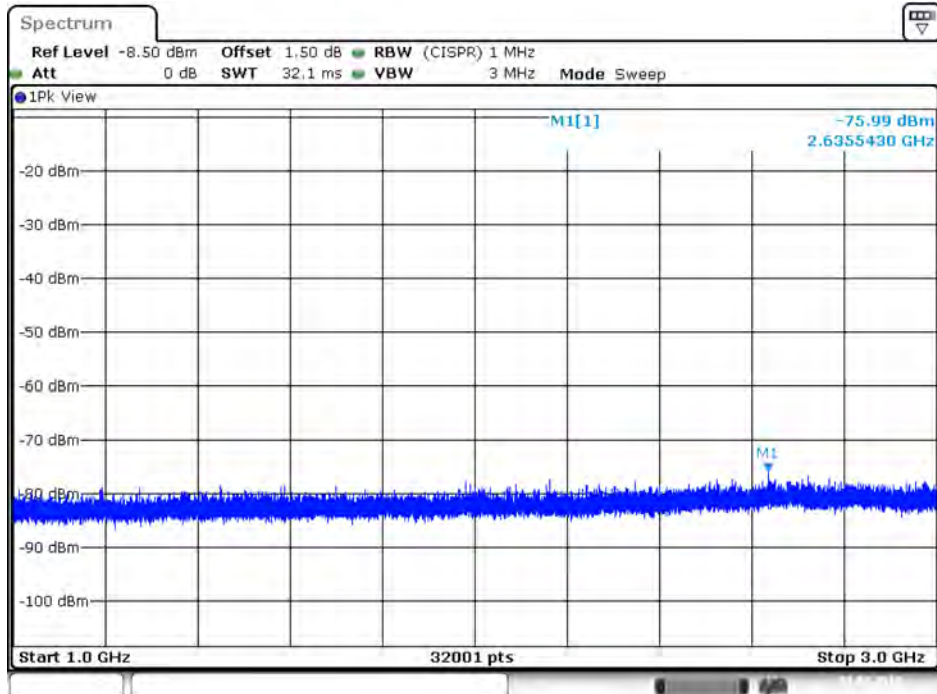
Plot on IEEE 802.11ac Nss1 MCS0 VHT20 / 5320 MHz / Peak / Port 1 / 1GHz~3GHz
