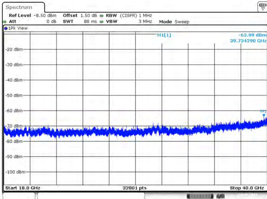
Plot on IEEE 802.11ac Nss1 MCS0 VHT20 / 5500 MHz / Peak / Port 1 / 18GHz~40GHz
