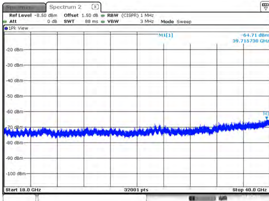
Plot on IEEE 802.11ac Nss1 MCS0 VHT20 / 5260 MHz / Peak / Port 1 / 18GHz~40GHz
