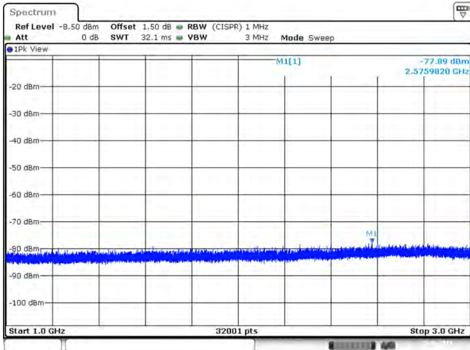
Plot on IEEE 802.11ac Nss1 MCS0 VHT80 / 5610 MHz / Peak / Port 1 / 1GHz~3GHz
