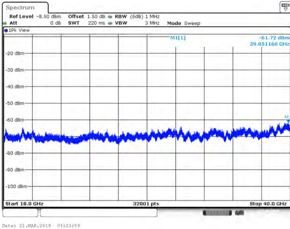
Plot on IEEE 802.11ac Nss1 MCS0 VHT80 / 5290 MHz / Peak / Port 1 / 18GHz~40GHz
