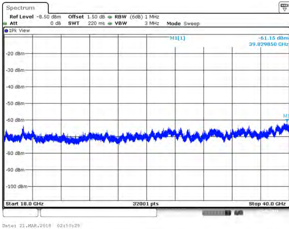
Plot on IEEE 802.11ac Nss1 MCS0 VHT80 / 5290 MHz / Peak / Port 2 / 18GHz~40GHz
