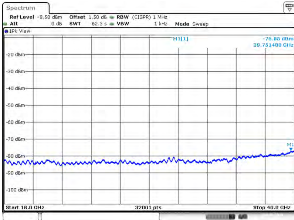
Plot on IEEE 802.11ac Nss1 MCS0 VHT80 / 5530 MHz / Average / Port 1 / 18GHz~40GHz
