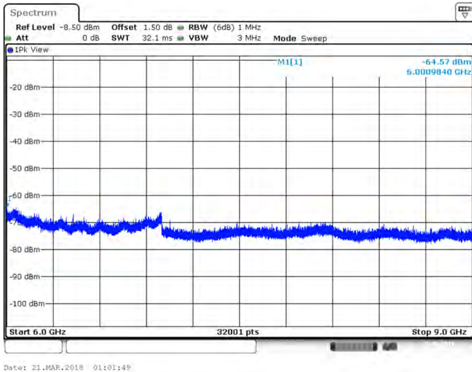
Plot on IEEE 802.11ac Nss1 MCS0 VHT80 / 5290 MHz / Peak / Port 2 / 6GHz~9GHz
