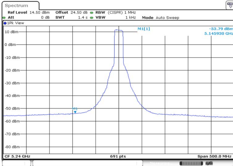
Plot on IEEE 802.11ac Nss1 MCS0 VHT20 / 5240 MHz / Average / Port 2
