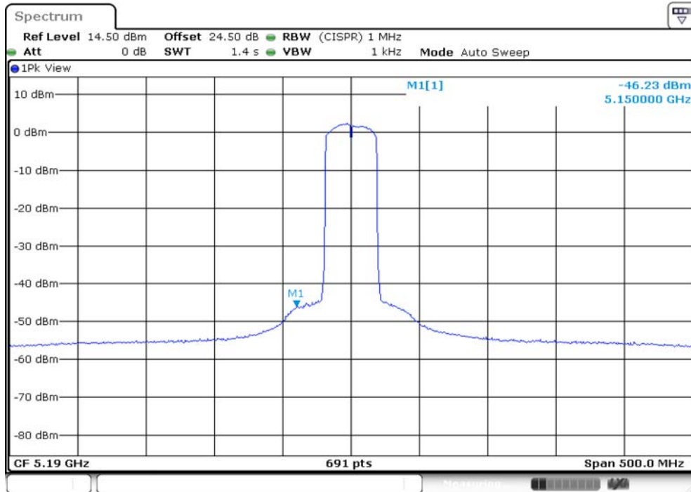
Plot on IEEE 802.11ac Nss1 MCS0 VHT40 / 5190 MHz / Average / Port 2
