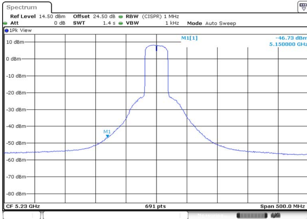
Plot on IEEE 802.11ac Nss1 MCS0 VHT40 / 5230 MHz / Average / Port 2
