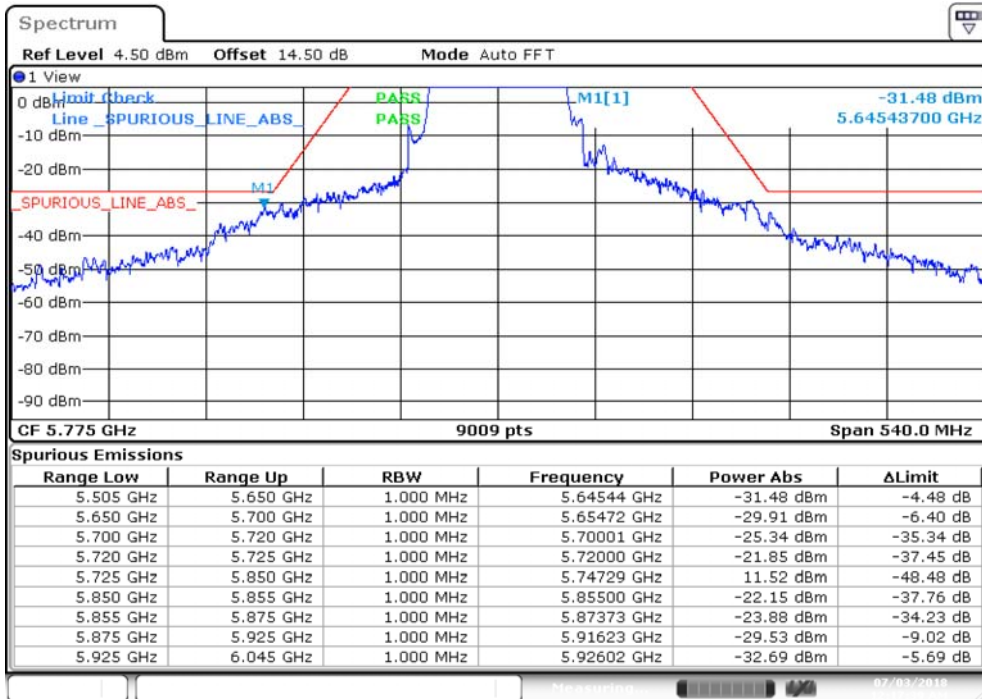
Plot on IEEE 802.11ac Nss1 MCS0 VHT80 / 5775 MHz / Peak / Port 2
