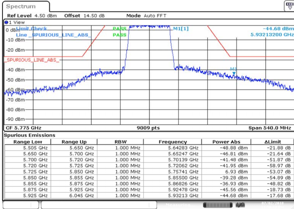
Plot on IEEE 802.11ac Nss1 MCS0 VHT80 / 5775 MHz / Peak / Port 1
