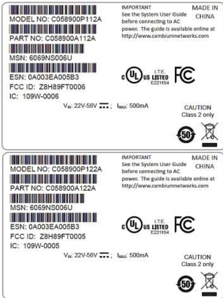
Figure 64 FCC and IC certifications on 5 GHz product labels
