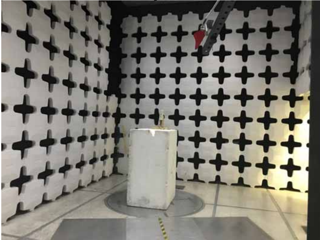
Test Setup for Radiated Emissions above 1-18GHz – Horizontal Polarization
