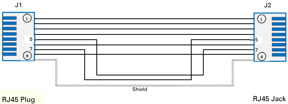
Figure 31 CMM4 power adapter cabling diagram
