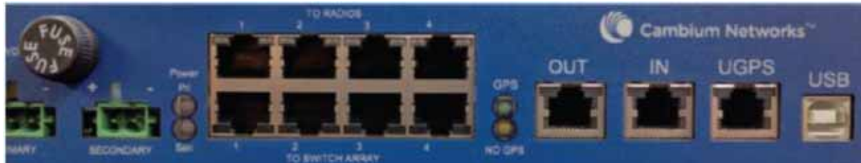
Figure 28 Injector Module
