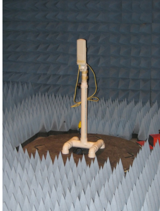
Radiated Above 1 GHz with Integral Patch Antenna - Front
