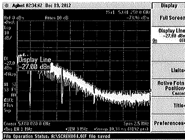
Plot 4: 20MHz RF Channel 5660 MHz
