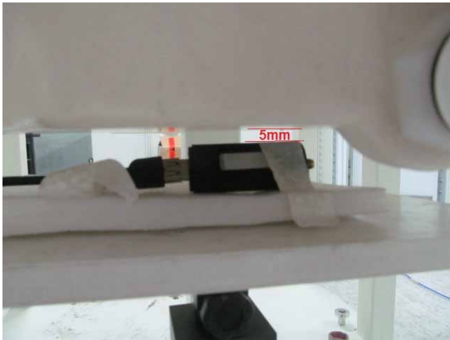
PCB Antenna (Vertical Front)
