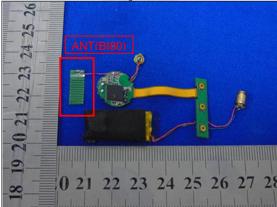
The original antenna
