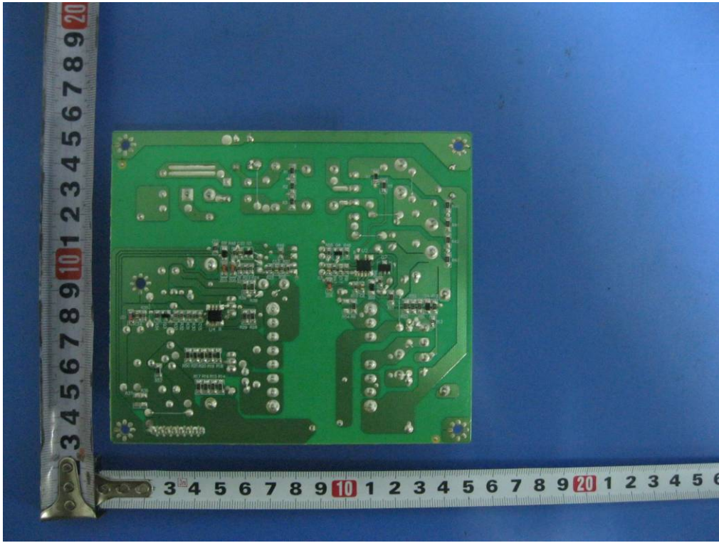
EUT -PCB Rear View 1
