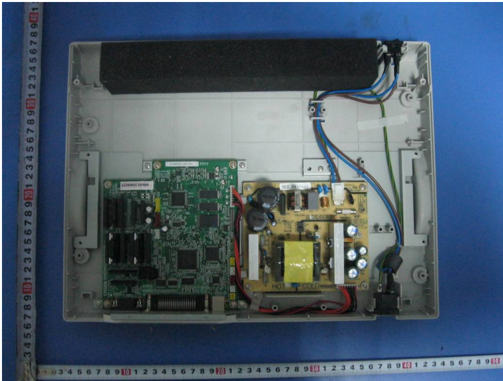
EUT – Uncover Top View
