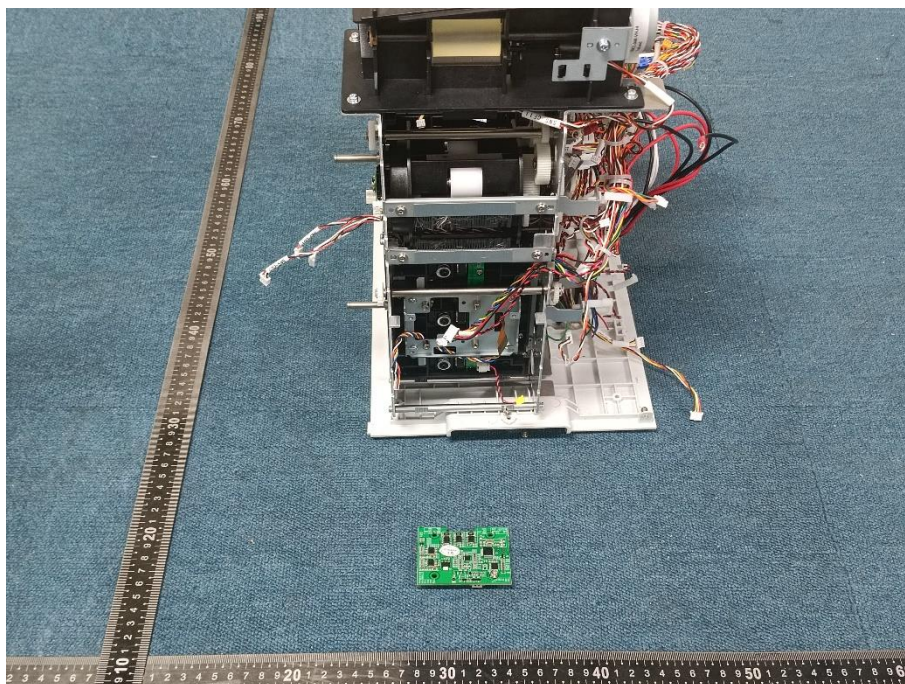
EUT UNCOVER VIEW 14
