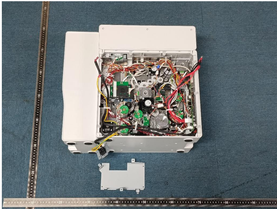
EUT UNCOVER VIEW 11
