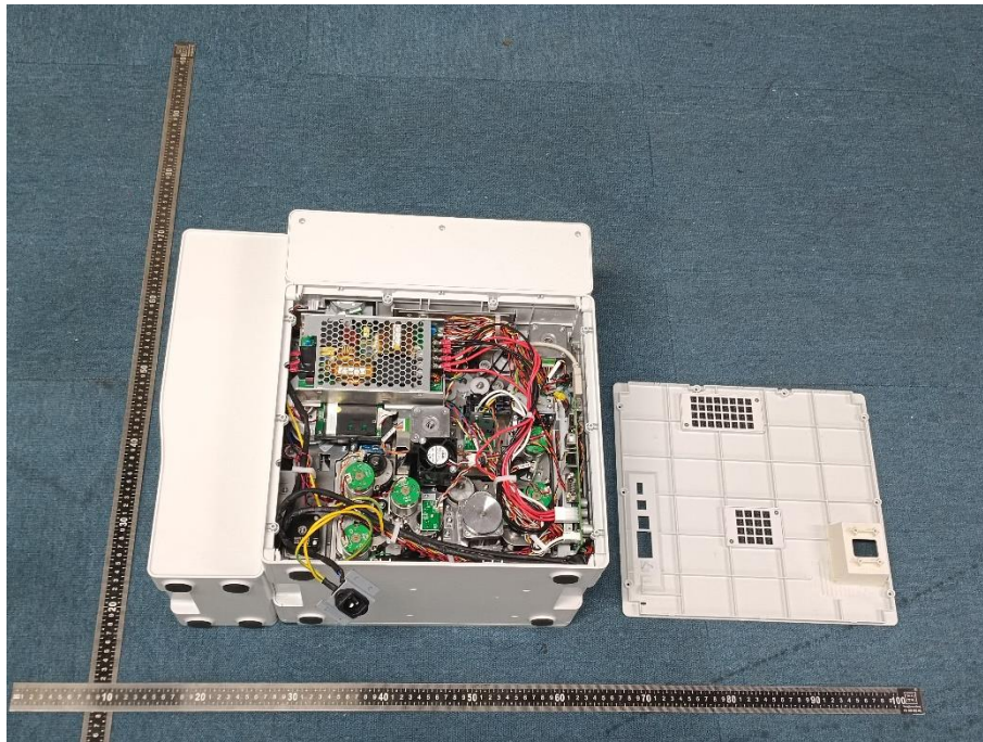
EUT UNCOVER VIEW 13
