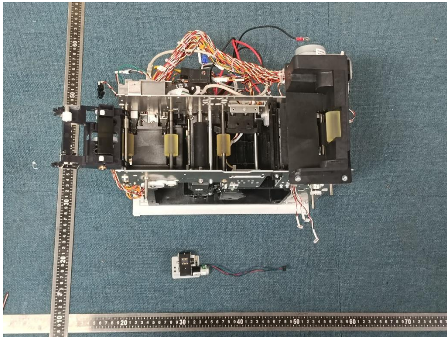
EUT UNCOVER VIEW 15
