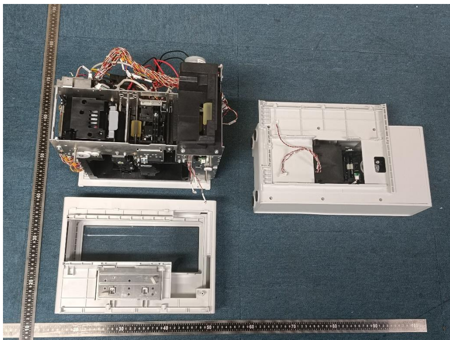
EUT UNCOVER VIEW 16
