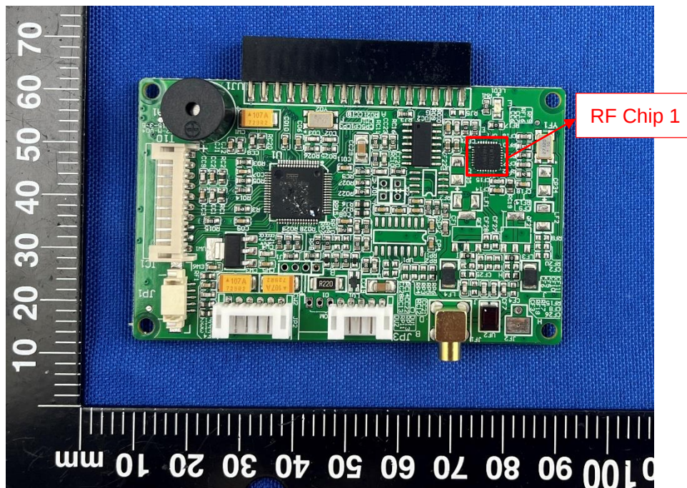
SECONDARY BOARD 1 TOP VIEW (RFID-1)
