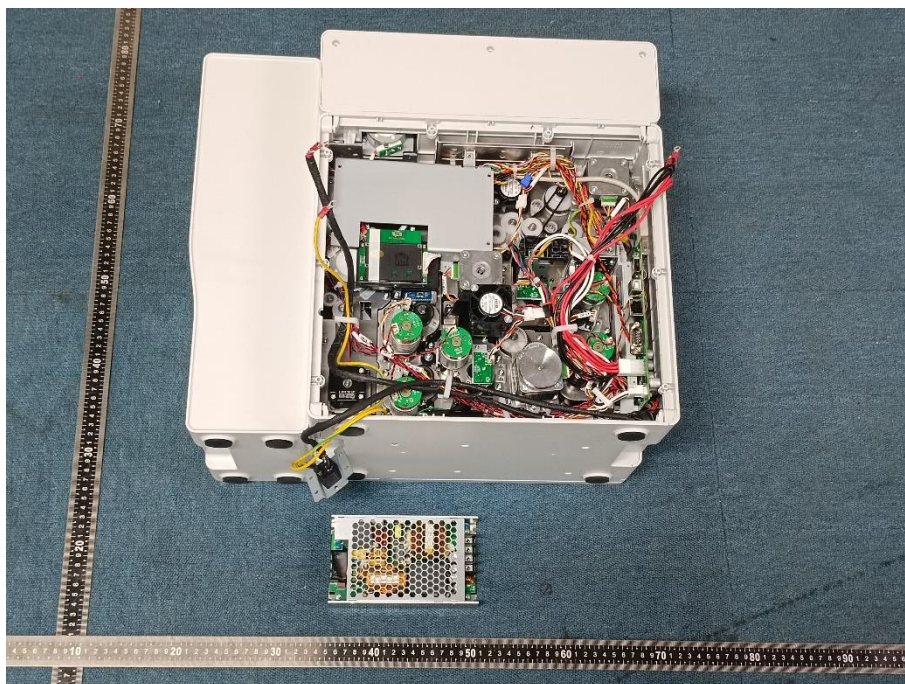
EUT UNCOVER VIEW 12
