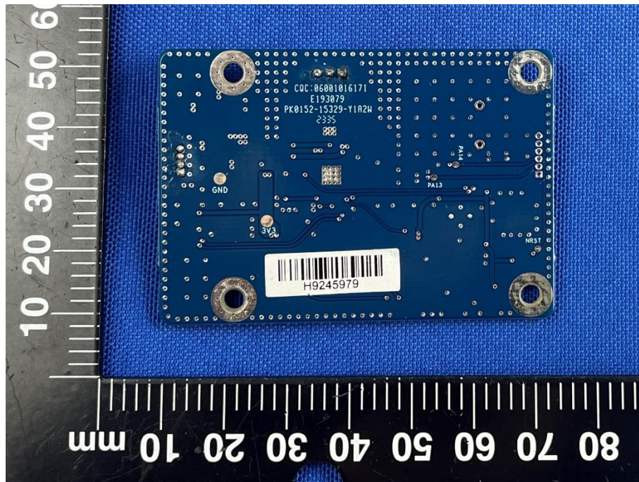
SECONDARY BOARD 3 REAR VIEW (RFID-3)
