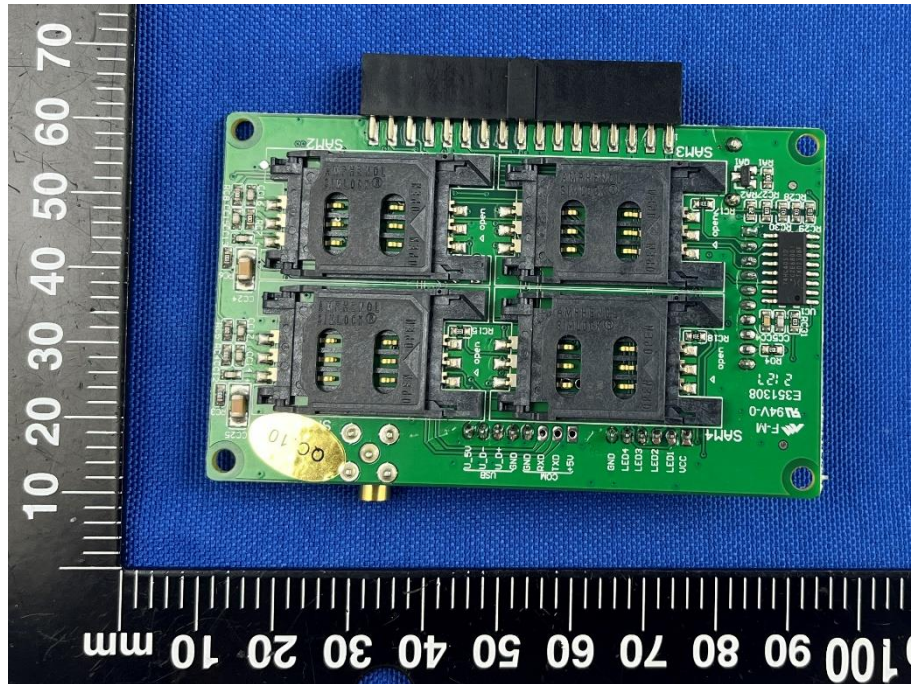
SECONDARY BOARD 1 REAR VIEW (RFID-1)
