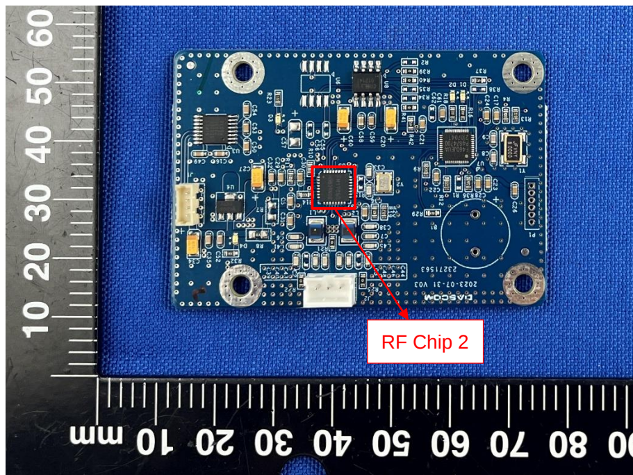
SECONDARY BOARD 2 TOP VIEW (RFID-2)
