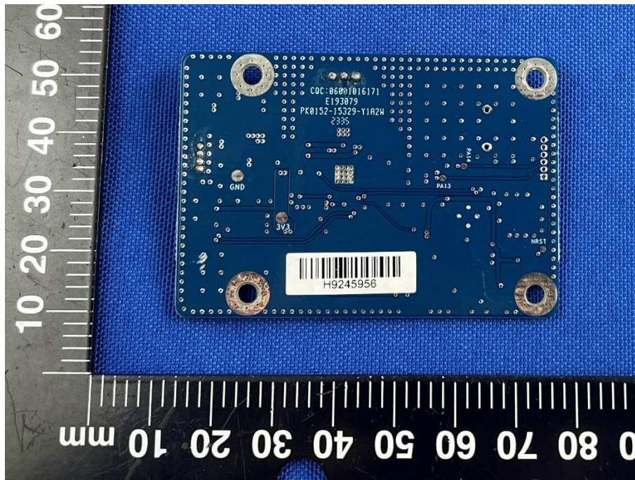
SECONDARY BOARD 2 REAR VIEW (RFID-2)
