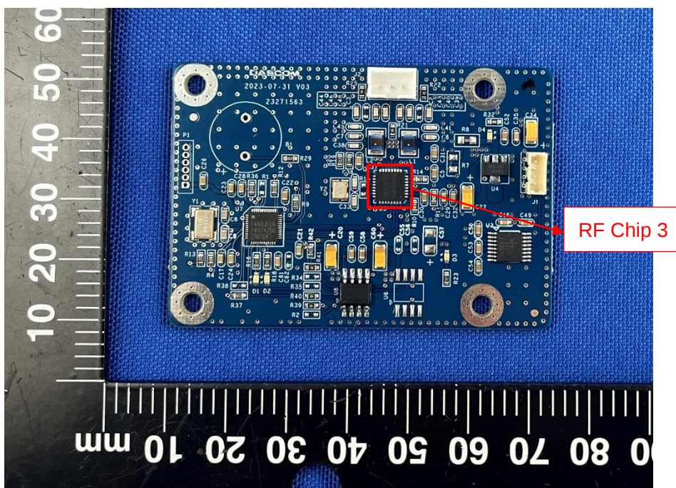
SECONDARY BOARD 3 TOP VIEW (RFID-3)
