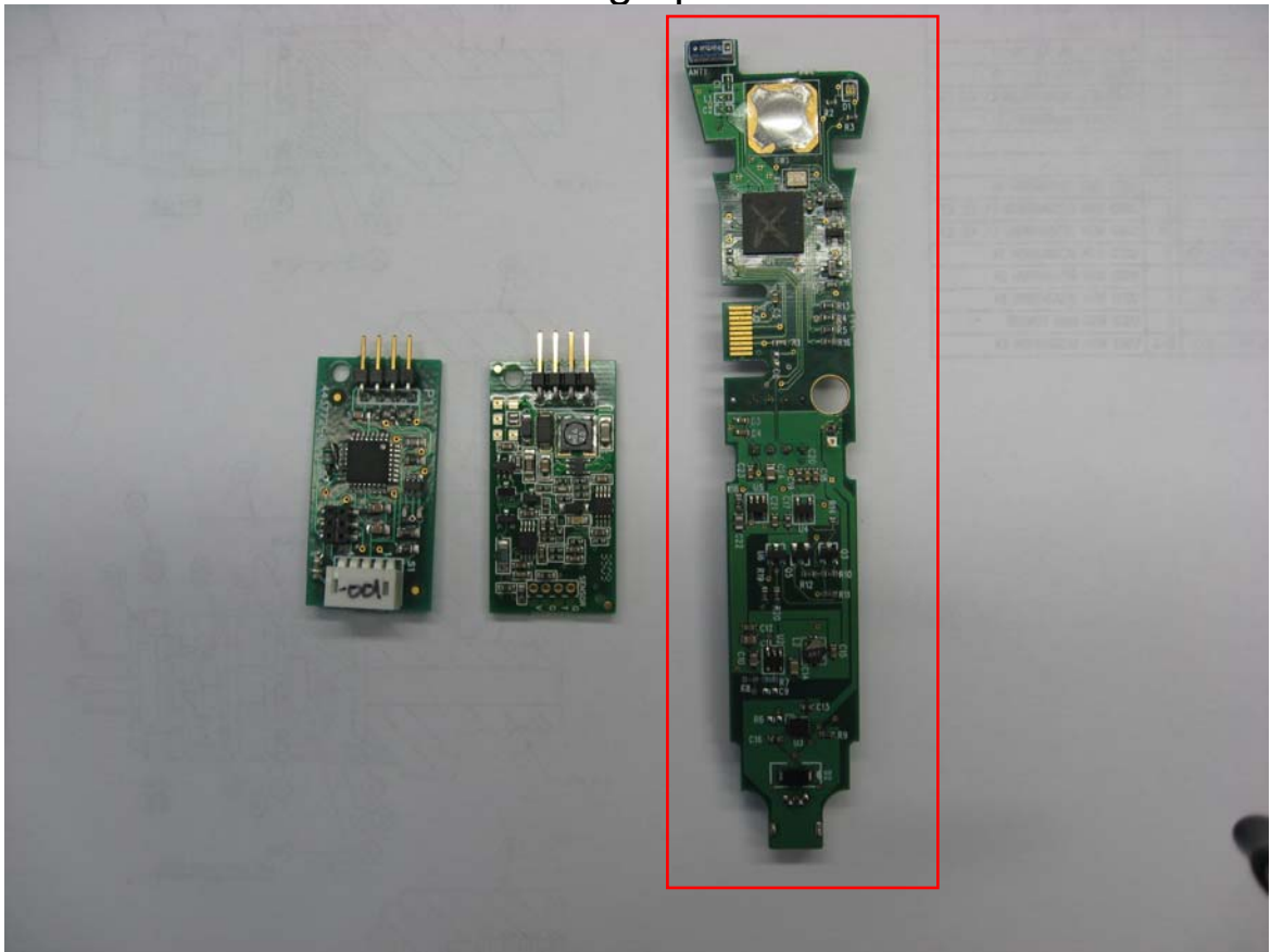
The module is the long board. This contains all of the RF circuitry. The small board is the sensor board.
