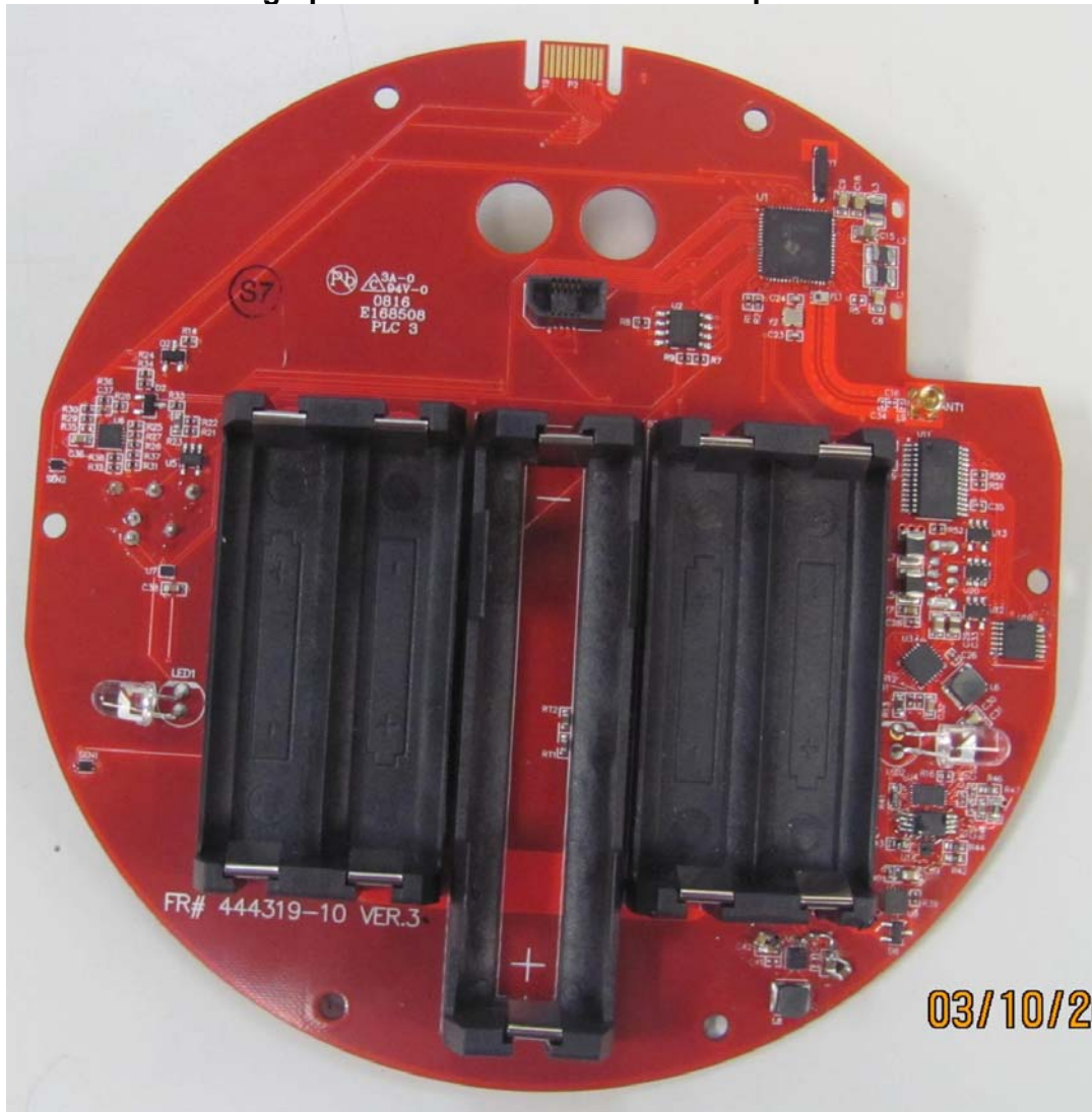
Photograph of Main Board with RF: Component Side
