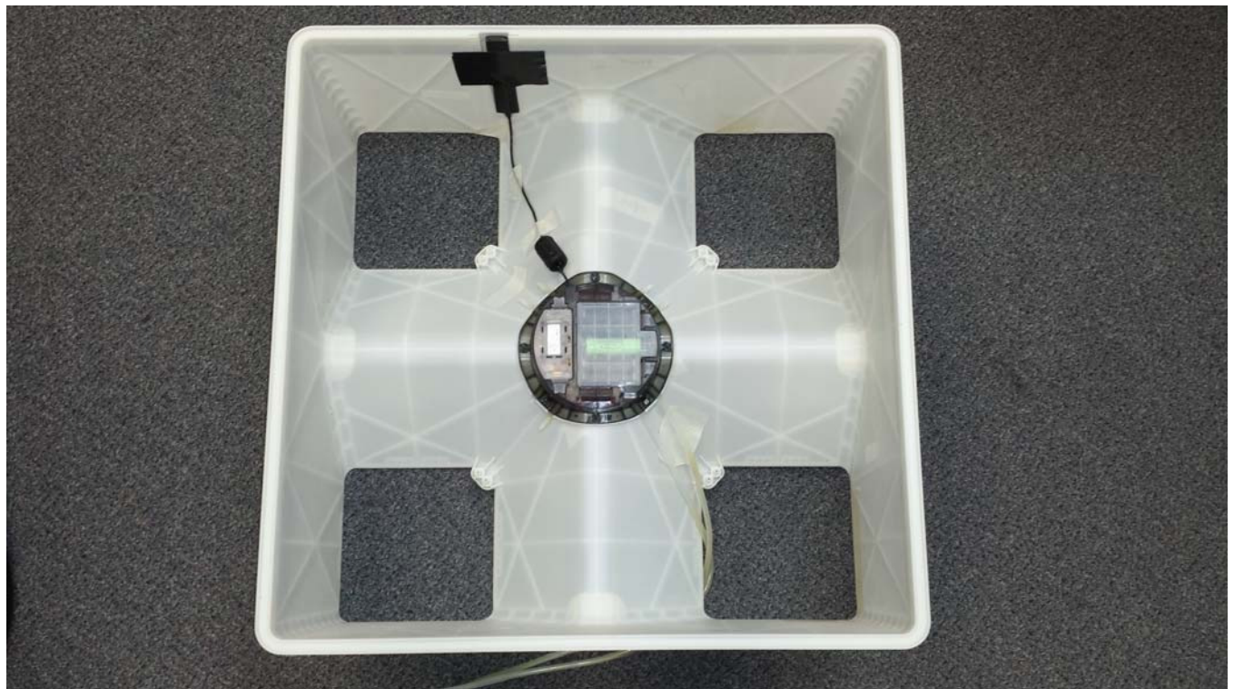
This is the EUT with the antenna installed. This is the prototype plastic
