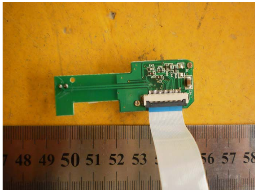
Camera PCB photograph of EUT
