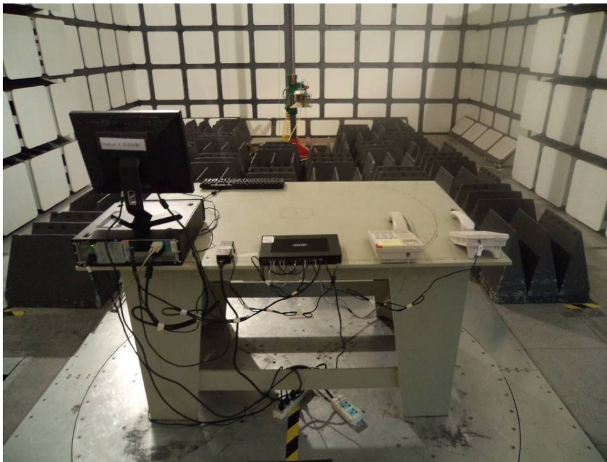
Radiated Emissions – Rear View (1-5 GHz)
