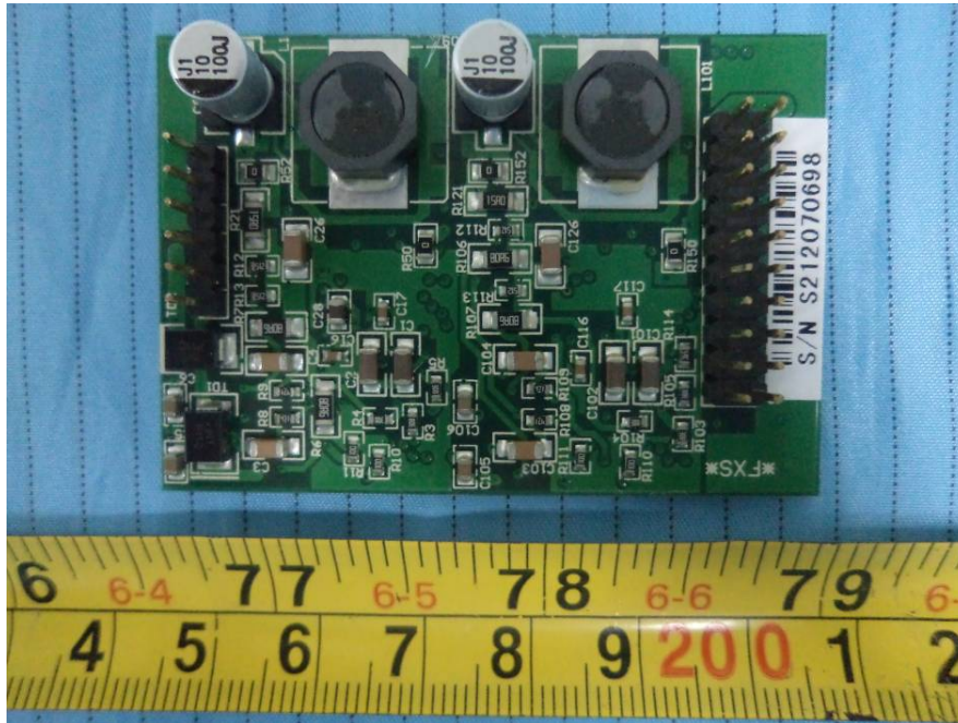
EUT- FXS Board Bottom View
