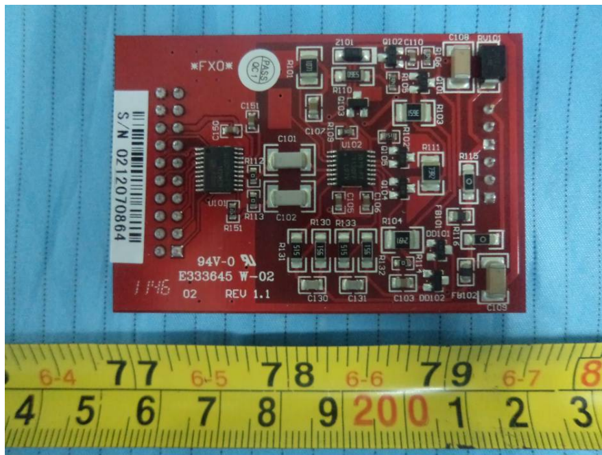
EUT – FXO Board Top View
