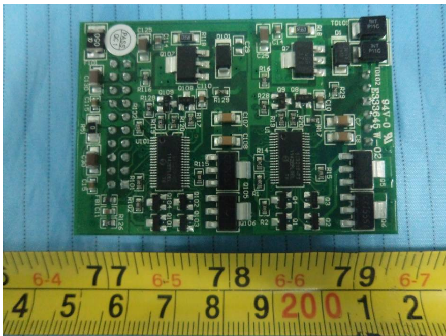
EUT – FXS Board Top View
