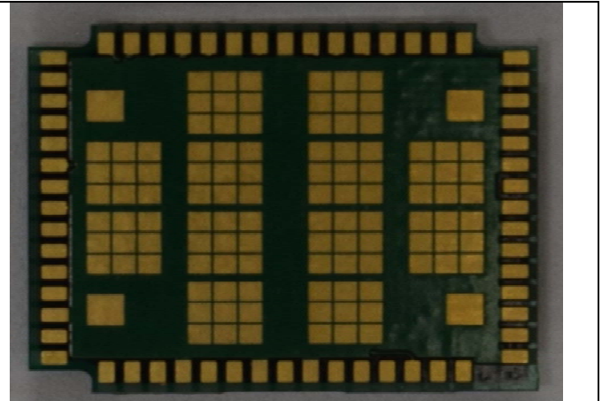
Radio Module - Bottom View
