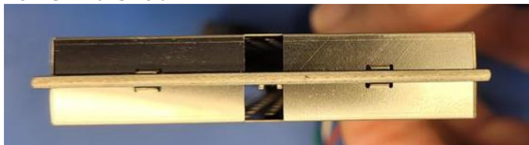
Side 4 View of PCB with Shield:
