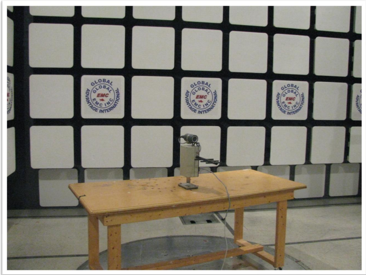
Figure 1 – EUT Emissions Setup
