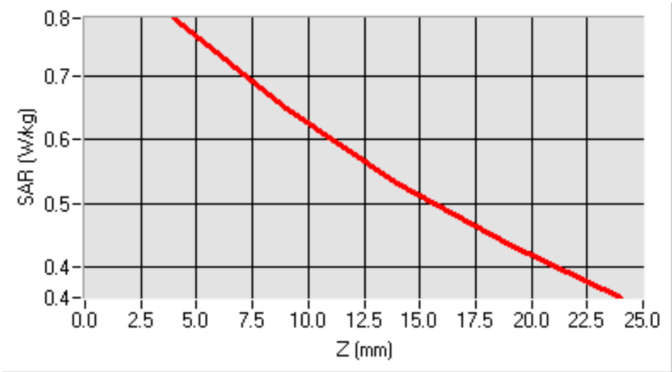
SAR, Z Axis Scan (X = -49, Y = -26)
