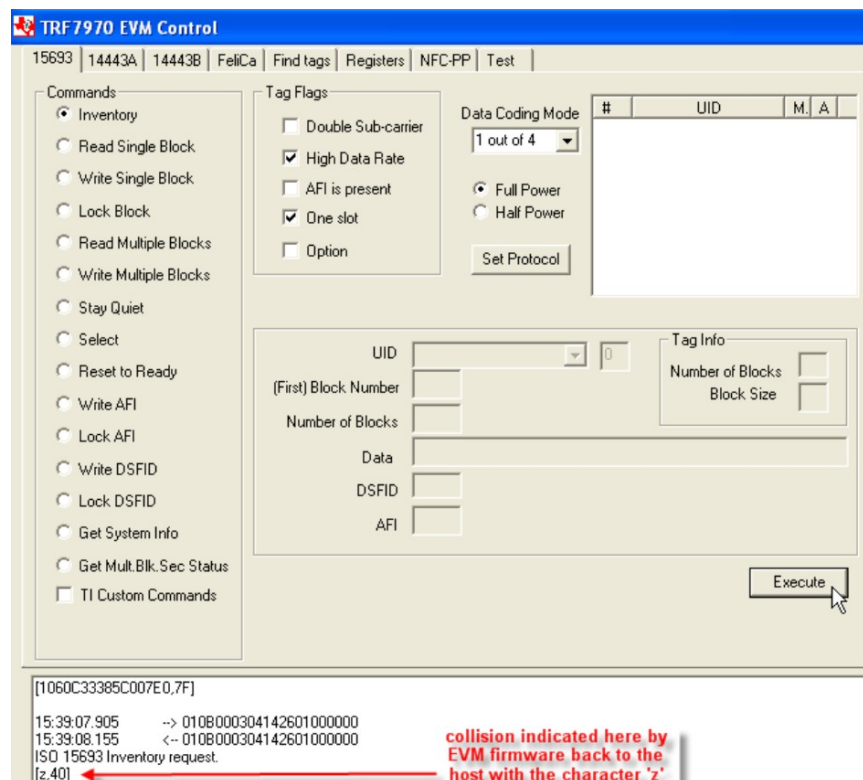
Figure 4. Single Slot Inventory Command (Two Tags in Field/Collision)
