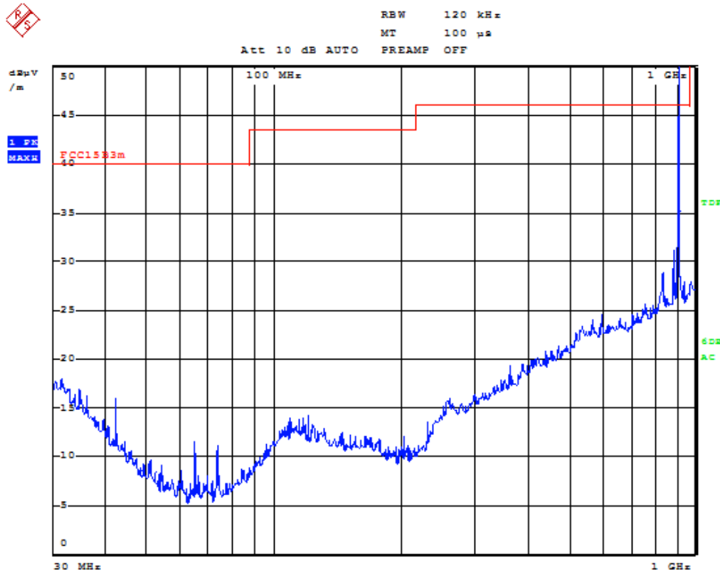
Figure 6. Spurious emissions, 30-1000 MHz, channel 915.0 MHz
