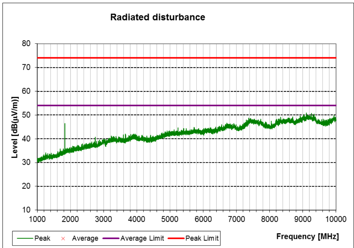
Figure 7. Spurious emissions, 1000-10000 MHz, channel 915.0 MHz
