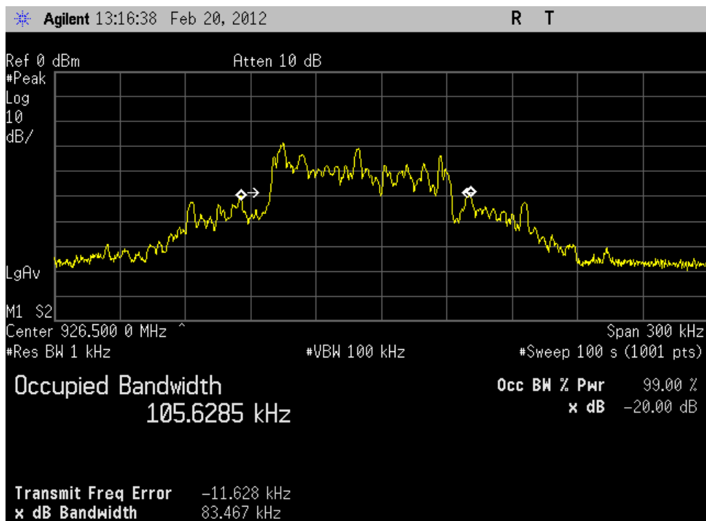
Figure 10. 20 dB bandwidth, channel 926.5 MHz.
