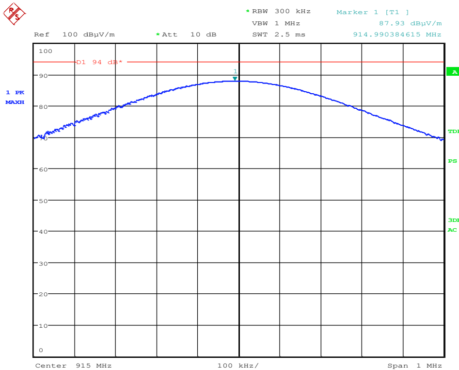
Figure 2. Fundamental output power, peak detector, channel 915.0 MHz
