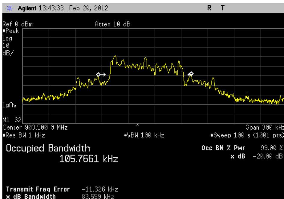
Figure 8. 20 dB bandwidth, channel 903.5 MHz.
