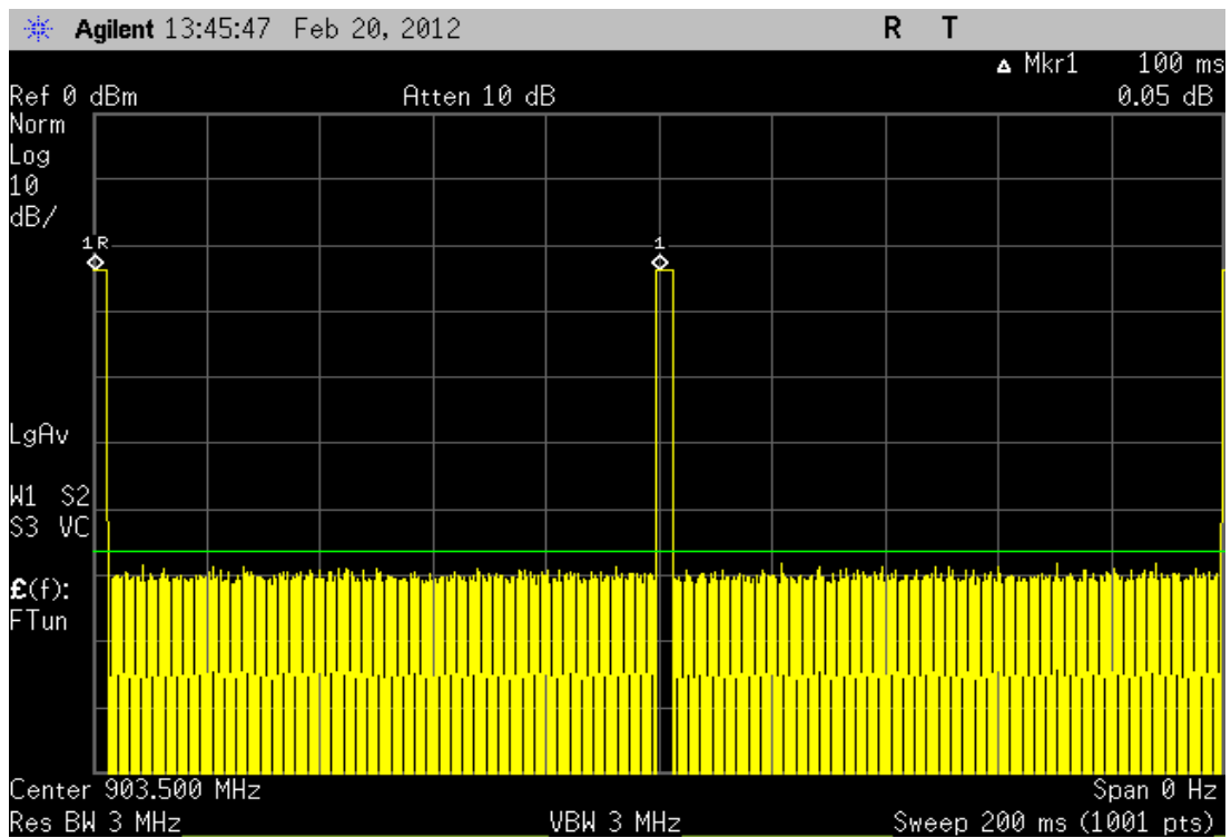
Figure 11. 100ms plot, channel 903.5 MHz.
