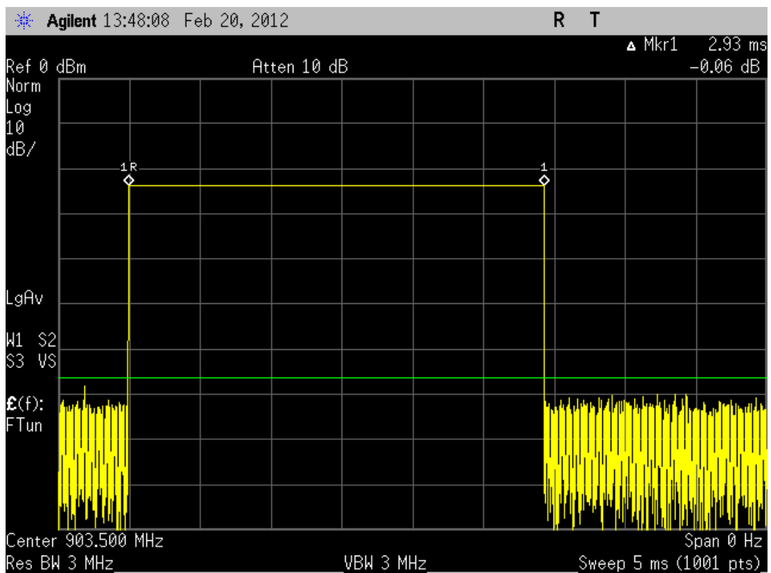
Figure 12. 5 ms plot, channel 903.5 MHz.
