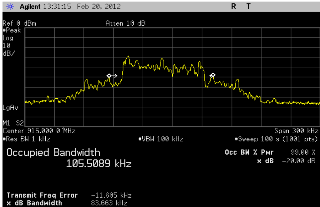
Figure 9. 20 dB bandwidth, channel 915.0 MHz.
