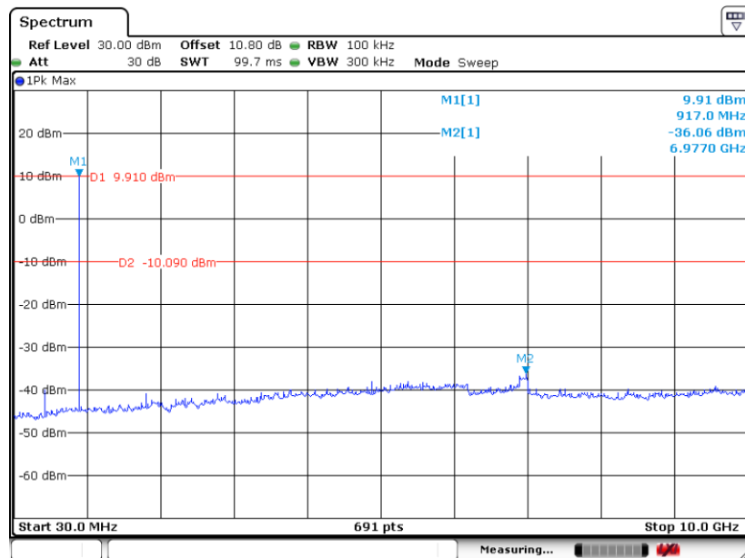
CSE Plot on Ch 65 between 30MHz ~ 10 GHz
