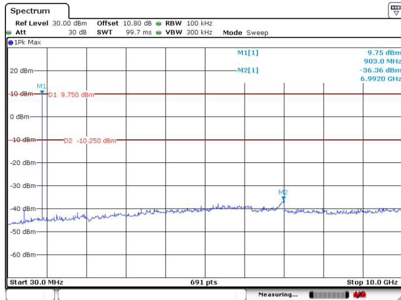
CSE Plot on Ch 01 between 30MHz ~10 GHz
