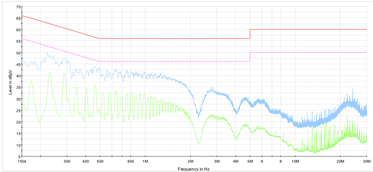
Conducted emissions on AC line, phase — CISPR 22 Mains QP Class B - - - CISPR 22 Mains AV Class B — Preview Result 1-PK+ — Preview Result 2-AVG
