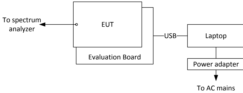
Figure 3.6-1: Setup diagram
