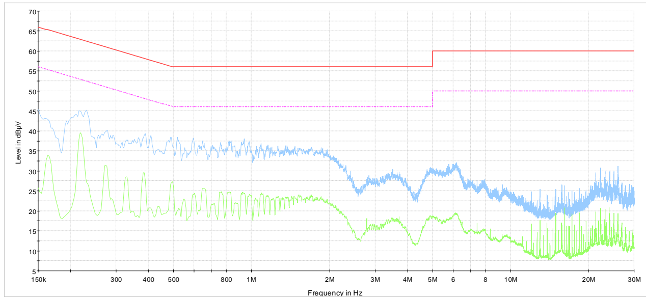
Conducted emissions on AC line, neutral — CISPR 22 Mains QP Class B - - - CISPR 22 Mains AV Class B — Preview Result 1-PK+ — Preview Result 2-AVG
