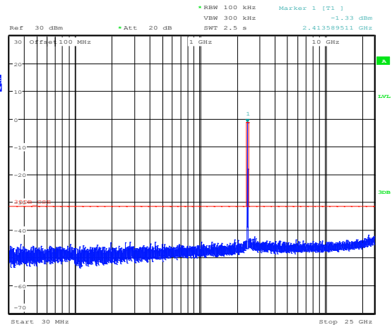
Figure 8.5-5: Conducted outside restricted bands spurious emissions for 802.11b, mid channel
