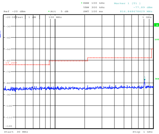
Figure 8.5-21: Conducted spurious emissions within restricted bands below 1 GHz for 802.11b, high channel
