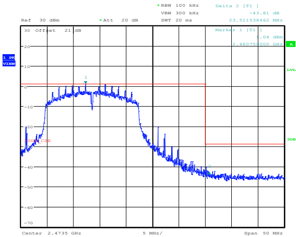
Figure 8.5-16: Conducted outside restricted bands band edge emissions for 802.11b, at 2.4835 GHz
