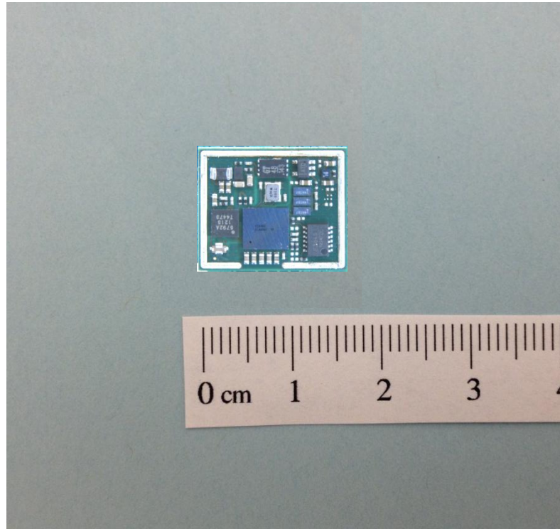
Internal Photo – CC3000MOD with shield removed
