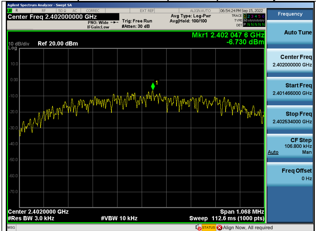
Test_Graph_LE1M_ANT1_2402_1Mbps_PSD
