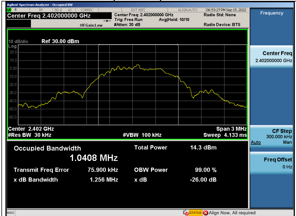
Test_Graph_LE1M_ANT1_2402_1Mbps_OBW
