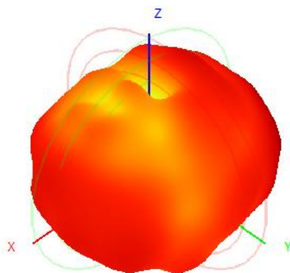
3-1 Antenna 3D Radiation Pattern
