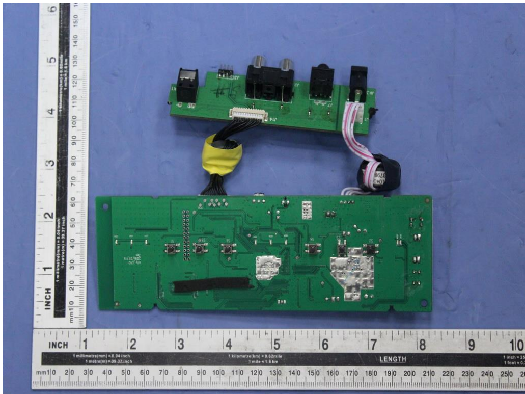
Fig. 4: Internal view
