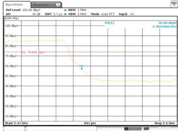
8-DPSK HIGH FREQUENCY BAND, PEAK
