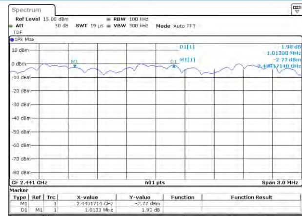
8-DPSK
