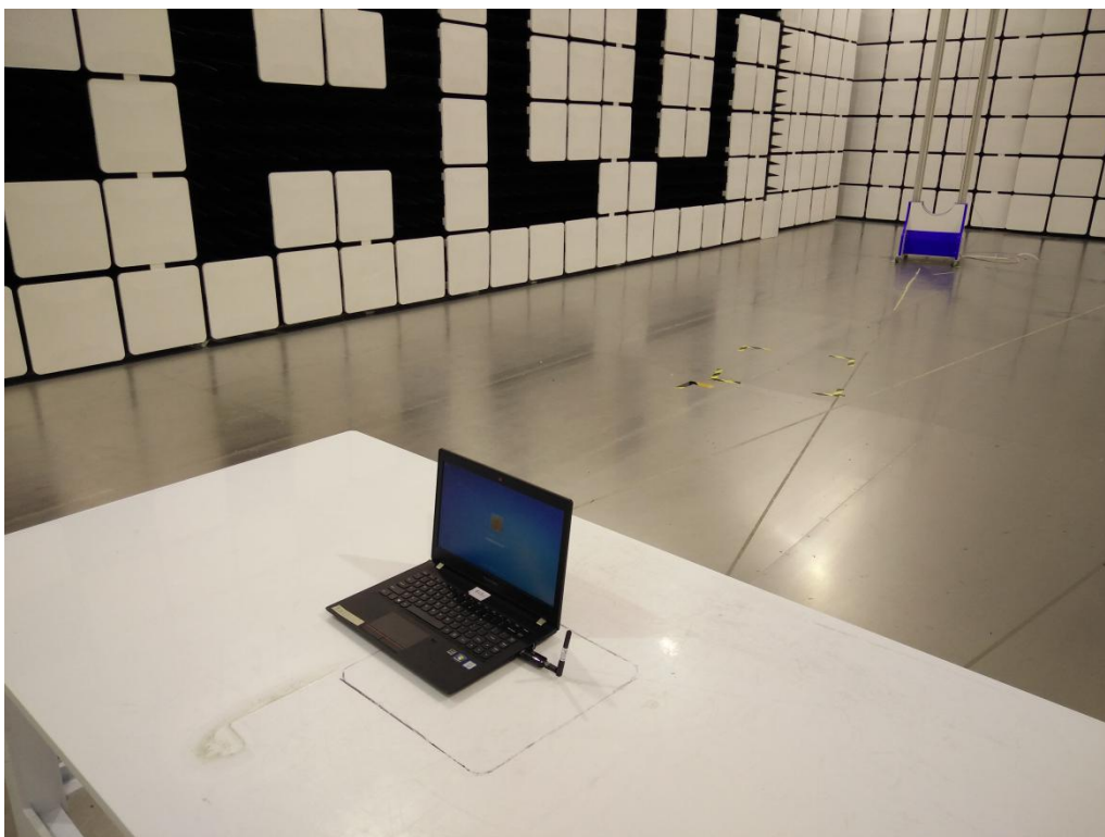
Radiated Test 2
