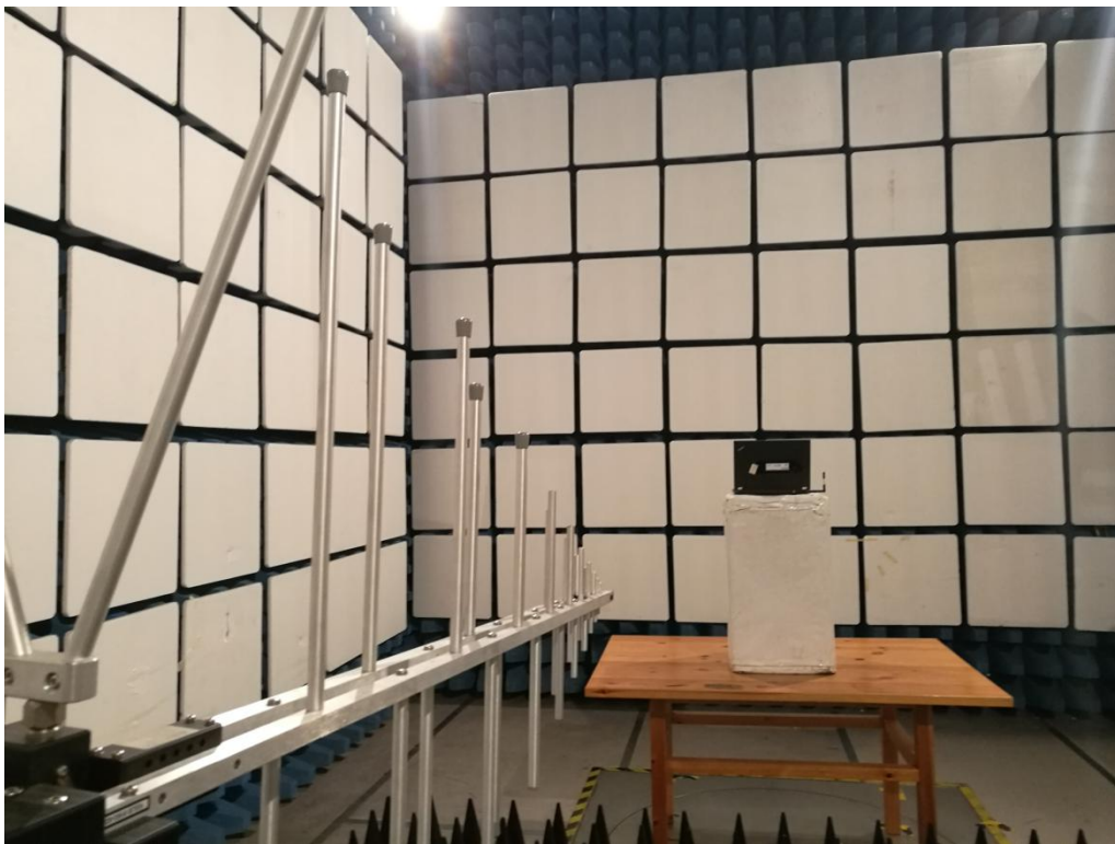
Radiated Test 4
