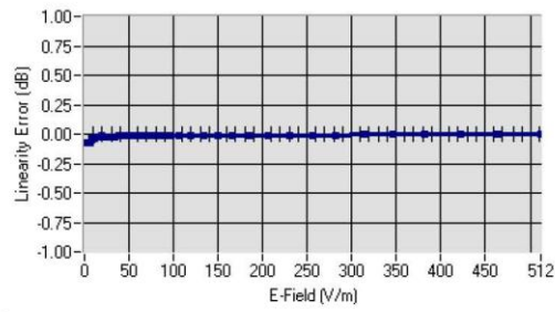
Linearity
