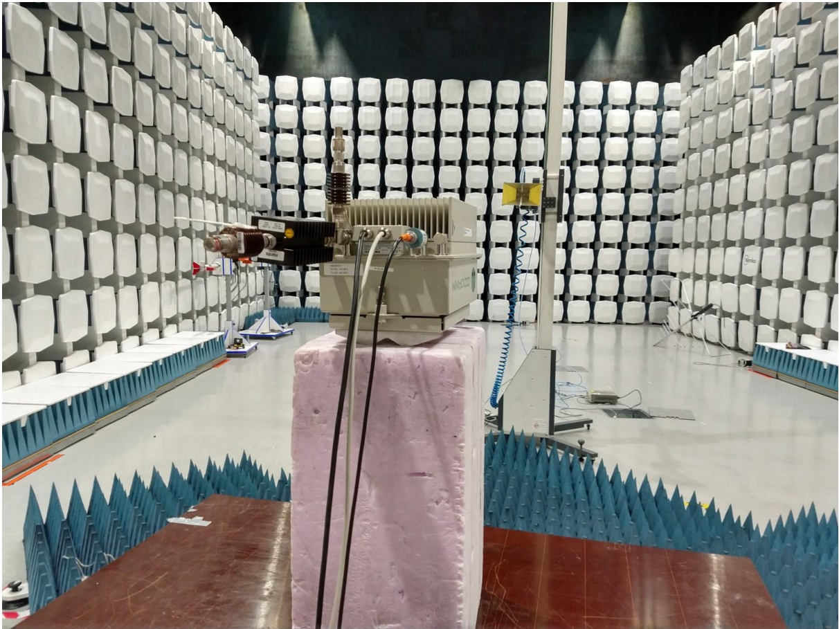
Radiated emissions 1 – 10GHz
