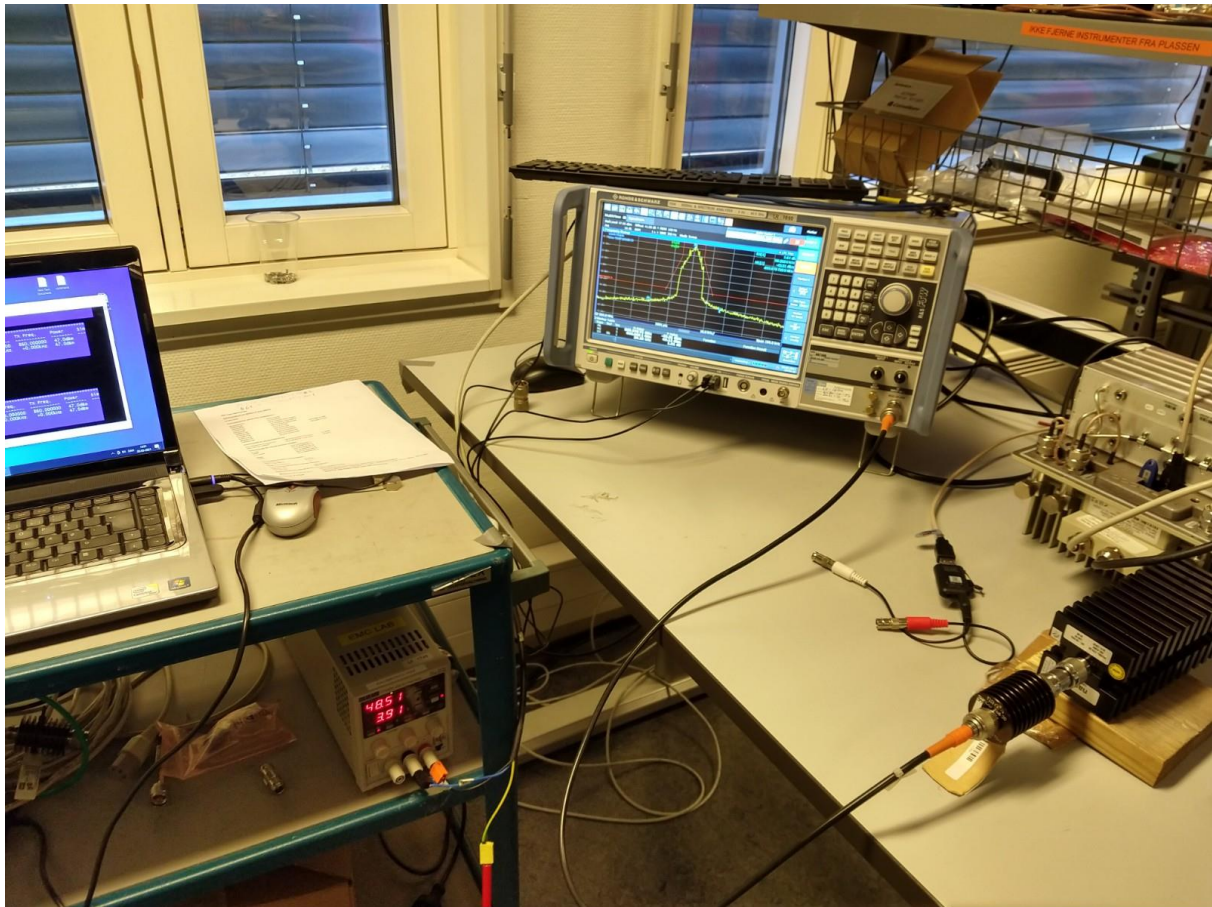
Conducted measurements
