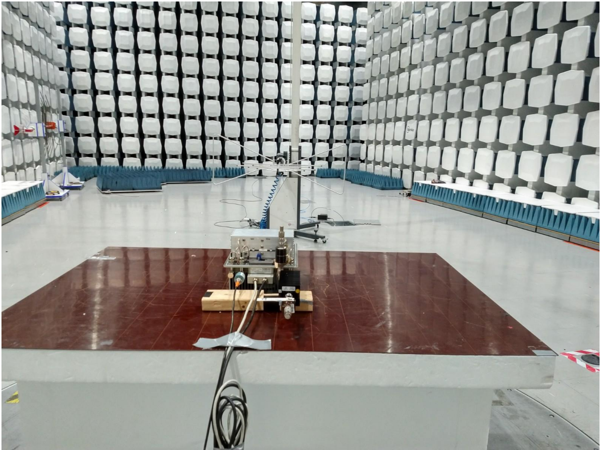
Radiated emissions 30 - 100MHz
