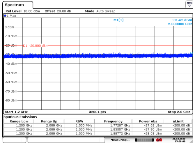
Figure 6.5-23: Conducted Spurious Emissions above 1.2 GHz, Tx @mid channel 50W 11Kof3E modulation
