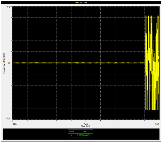
Figure 6.7-6: Transient Frequency behavior, Tx @ mid channel 6.25 k channel, switch OFF
