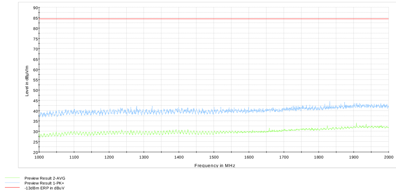
Figure 6.6-10: Cabinet Radiated Spurious Emissions above 1 GHz, Tx @ mid channel 50W 16KQF3E modulation
