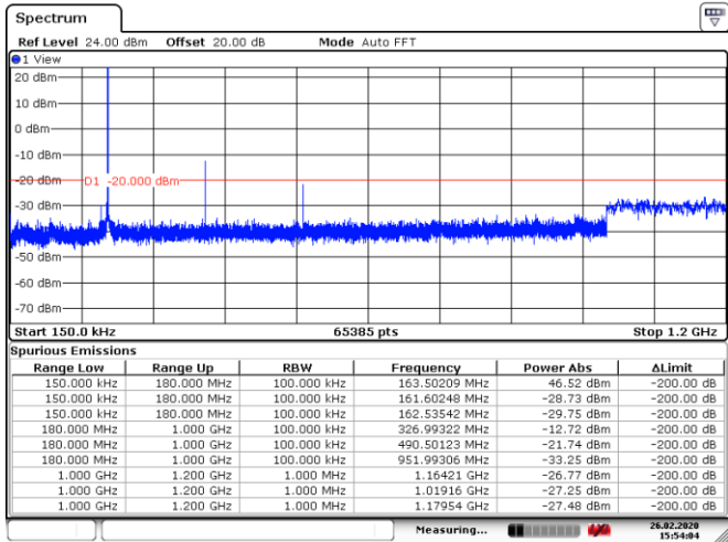
Figure 6.5-22: Conducted Spurious Emissions below 1.2 GHz, Tx @mid channel 50W 11Kof3E modulation
