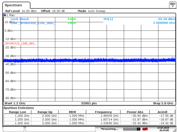
Figure 6.5-8: Conducted Spurious Emissions above 1.2 GHz, Tx @Low channel 25W 0.20TETRA modulation
