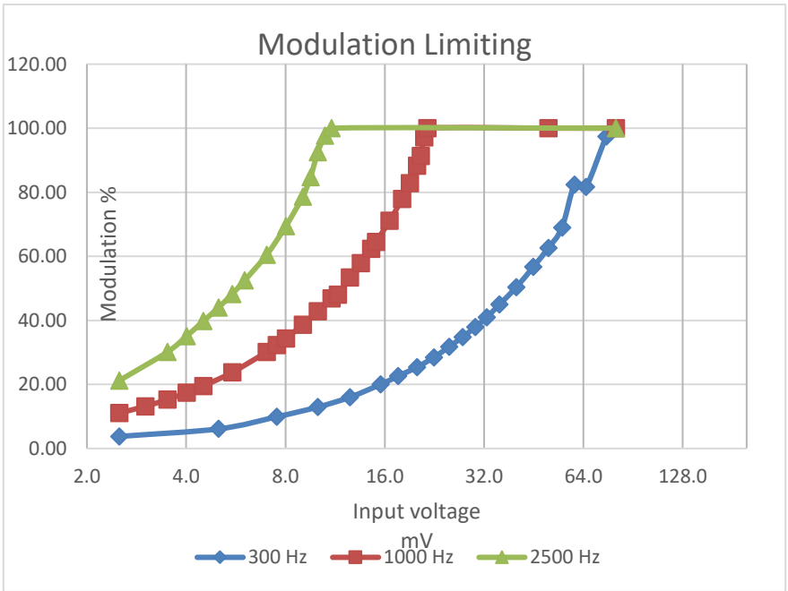
Figure 6.2-2: Modulation Limiting
