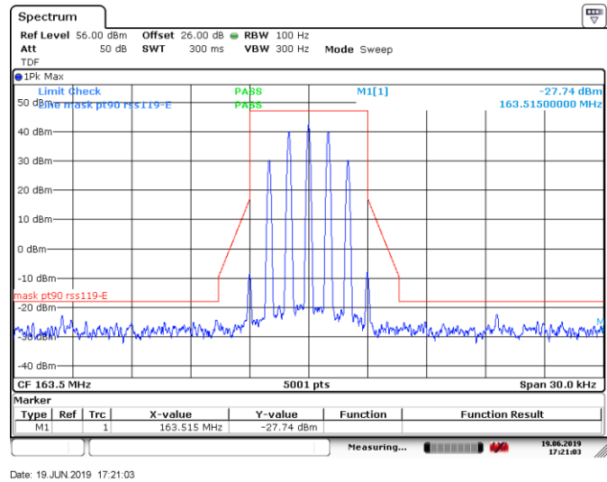
Figure 6.4-11: Mask e, Tx @mid channel 50W 6koF3E modulation
