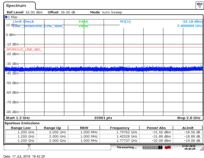
Figure 6.5-31: Conducted Spurious Emissions above 1.2 GHz, Tx @high channel 50W 7k60FXW modulation
