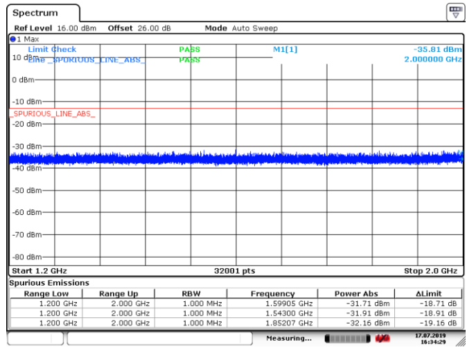
Figure 6.5-6: Conducted Spurious Emissions above 1.2 GHz, Tx @Low channel 50W 16Kof3E modulation
