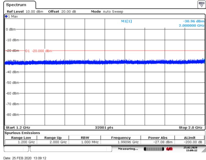
Figure 6.5-38: Conducted Spurious Emissions above 1.2 GHz, Tx @ high channel 50W 11K0F3E modulation
